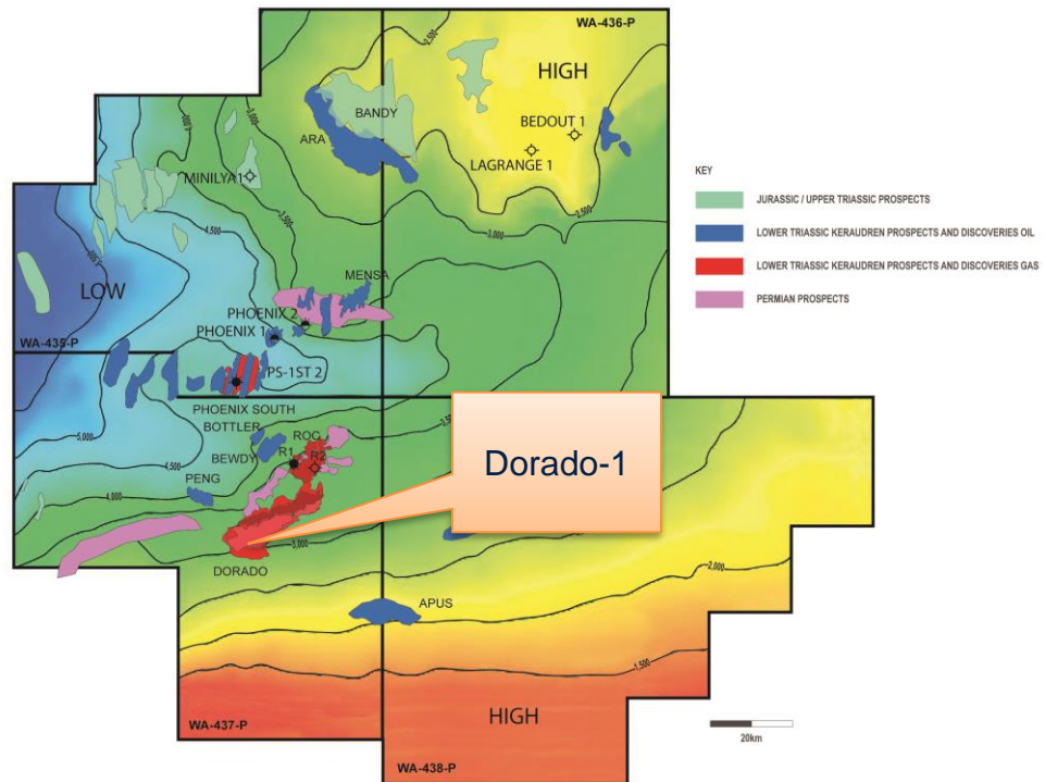
BASE TRIASSIC / TOP PERMIAN TIME STRUCTURE MAP (MILLISECONDS TWO WAY TIME)
