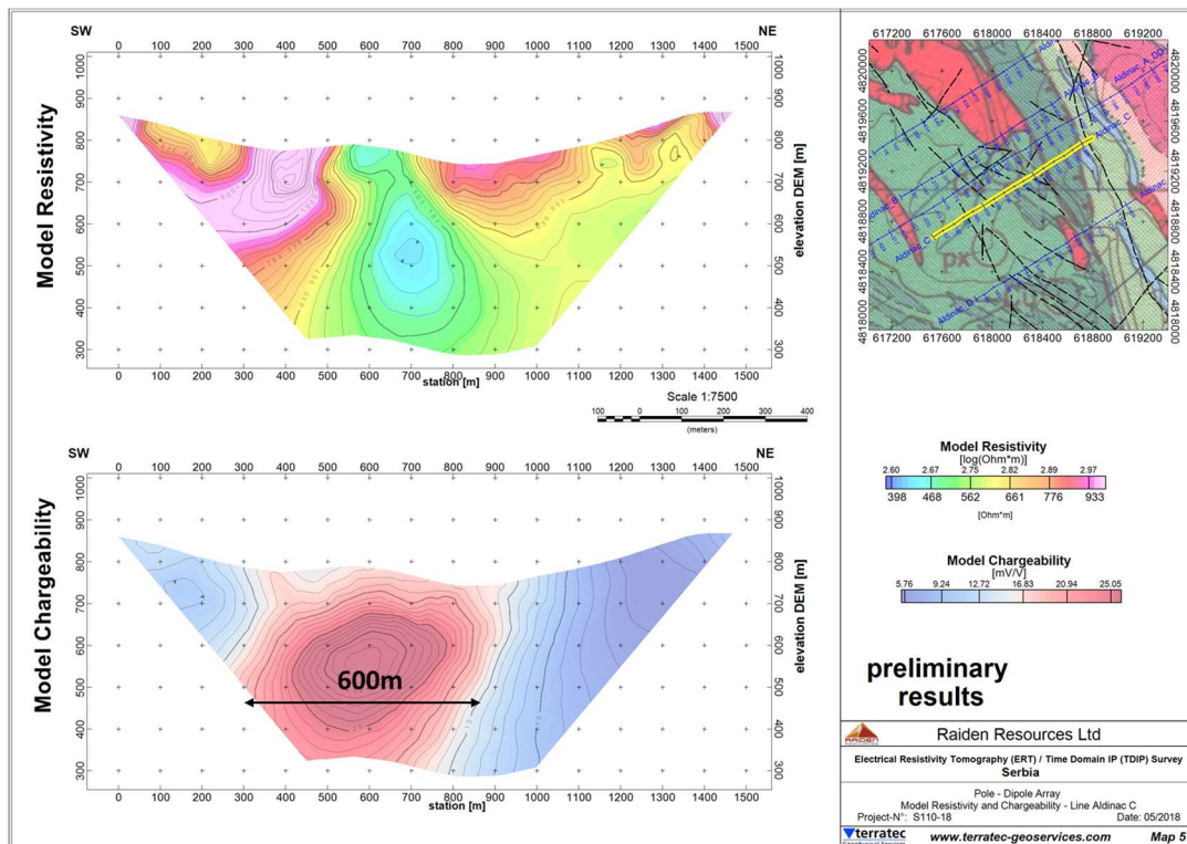
Figure 3 - Line C, which is located 200m south east of the original 2017 survey line AA, confirm the presence of an intense, 600m wide chargeability anomaly, with a vertical extent of 500m.
