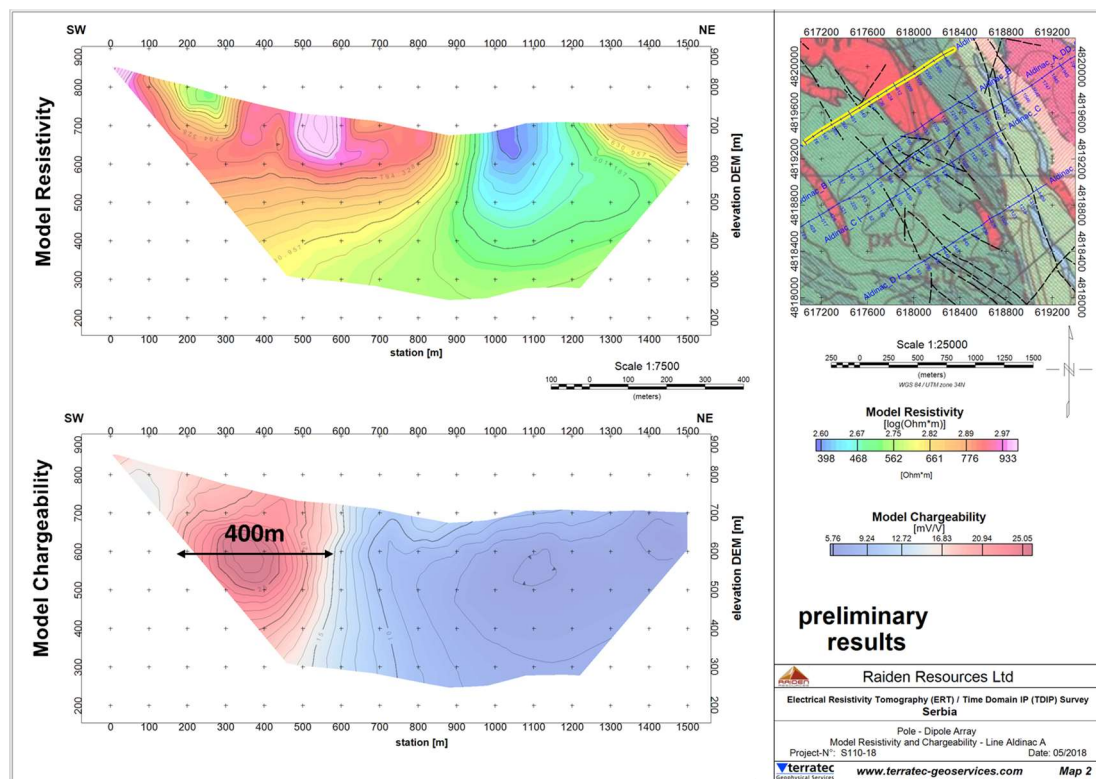
Figure 5 - IP line A, located 400m north west of Line B confirms the presence of a chargeability anomaly on the western side of the survey line. Anomaly is approximately 400m wide and has a vertical extends of 450m. The data indicates that the anomaly remains open along strike to the north west. The chargeability values may indicate the presence of disseminated sulphide mineralisation
