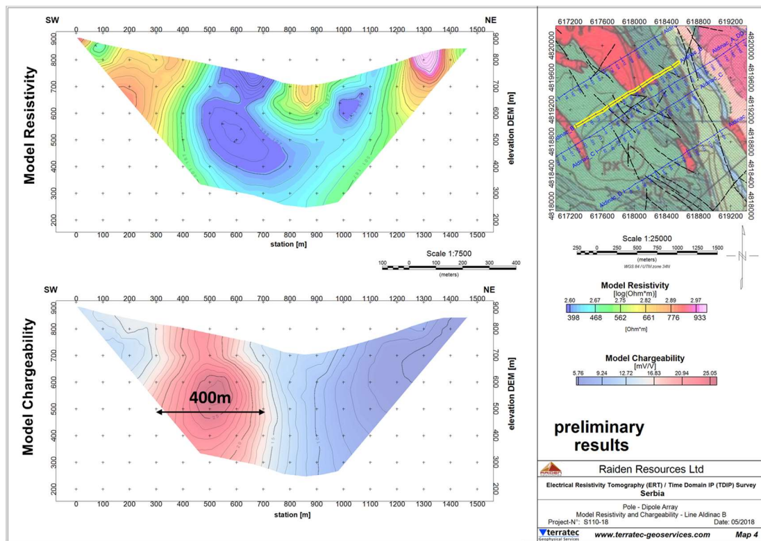
Figure 4 - Survey line B, located 600m north west of 2017 survey line, indicates a strong chargeability anomaly, 400m wide and with a 450m vertical extent. The chargeability anomaly is associated with low resistivity zone which may indicate the presence of massive and disseminated sulphide mineralisation
