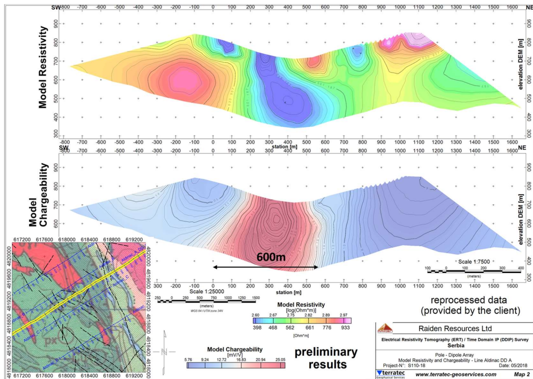
Figure 2 - Line AA, completed in 2017 and reinterpreted in context with recently acquired data. The anomaly is defined by a 600m wide intense chargeability anomaly, with a +450m vertical extent. The chargeability anomaly is coincidental with a resistivity depression, which may be interpreted as a zone of disseminated and massive sulphide mineralisation.
