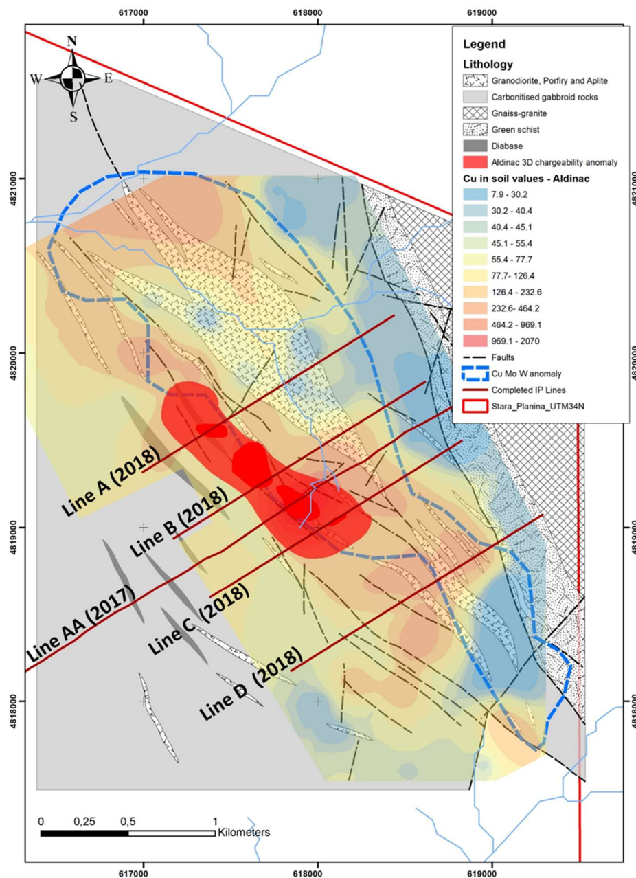
Figure 1 - Location of IP lines executed on the Aldinac anomaly. IP lines B, C and AA are centred over the highest Cu, Au and Mo values of the soil survey - Cu values represented as ppm. Lines C and B are parallel to the 2017 survey line (AA) and spaced 200 meters either side. Line A is approximately 400m north west of line B and line D is approximately 600m south east of line C.
