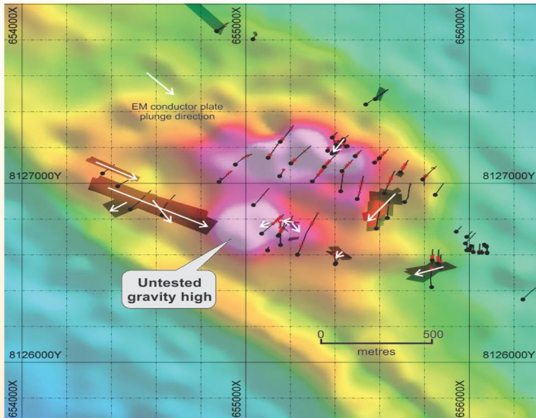
Figure 6. Plan of the Merlin Prospect showing recent ground gravity (Bouguer Anomaly) background image, highlighting the majority of modelled EM plates plunging towards an untested gravity high feature in the core of the Merlin Prospect.
