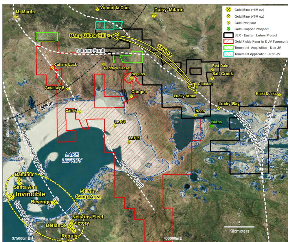
Figure 1 Lefroy Gold Project tenement plan showing Western Lefroy in red and Eastern Lefroy in black outline and proximity to St Ives. Lucky Strike, Capstan, Hang Glider Hill and recent tenement acquisitions are also highlighted.
