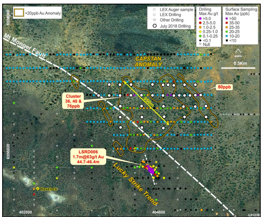
Figure 2 Capstan auger gold in auger anomaly sample points, completed drill holes and proximity to Lucky Strike.
