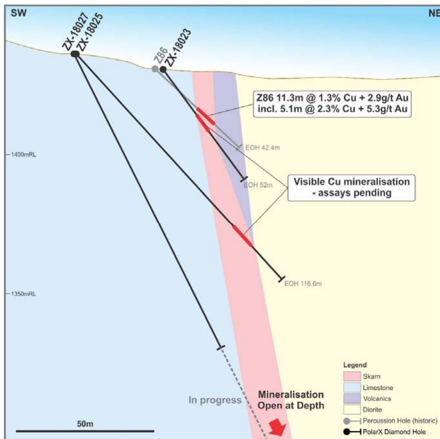
Figure 3 Cross-section showing relationship between holes ZX-18023 and ZX-18025 and historic percussion hole Z86.
