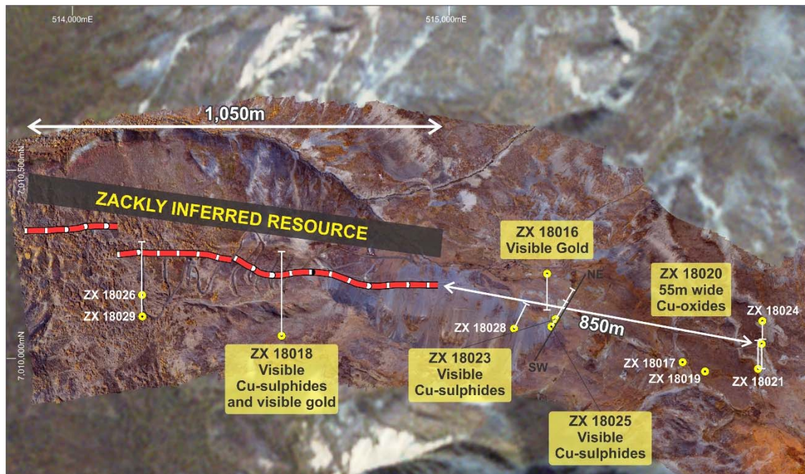
Figure 4. Drill hole plan for Zackly showing the 2017 surface trace of PolarX's inferred resource outline (red) and the 2018 drill holes collared to date (yellow) on detailed drone imagery.
