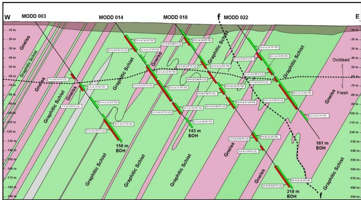
Figure 6. Cross section of the Caula Vanadium-Graphite Deposit
