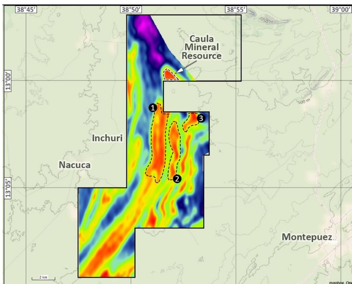
Figure 2. Potential of the larger Caula Project Area, SkyTEM Electromagnetic Signatures
