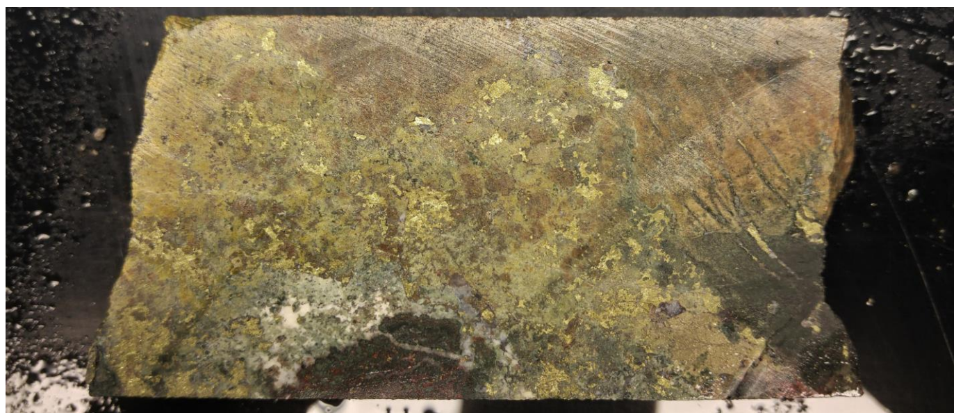
Figure 1: Drill core from FR18-004 with abundant sulphides comprising chalcopryite mineralisation within skarn at 282.3m
