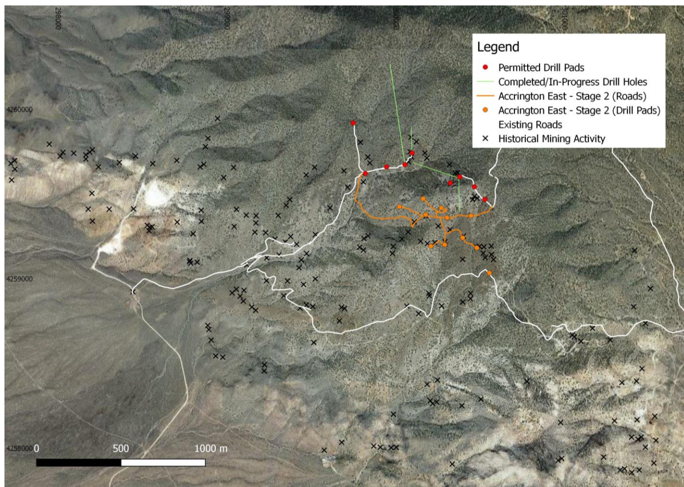
Figure 5: Accrington skarn with historical mining activity (shafts, adits, prospect pits).
