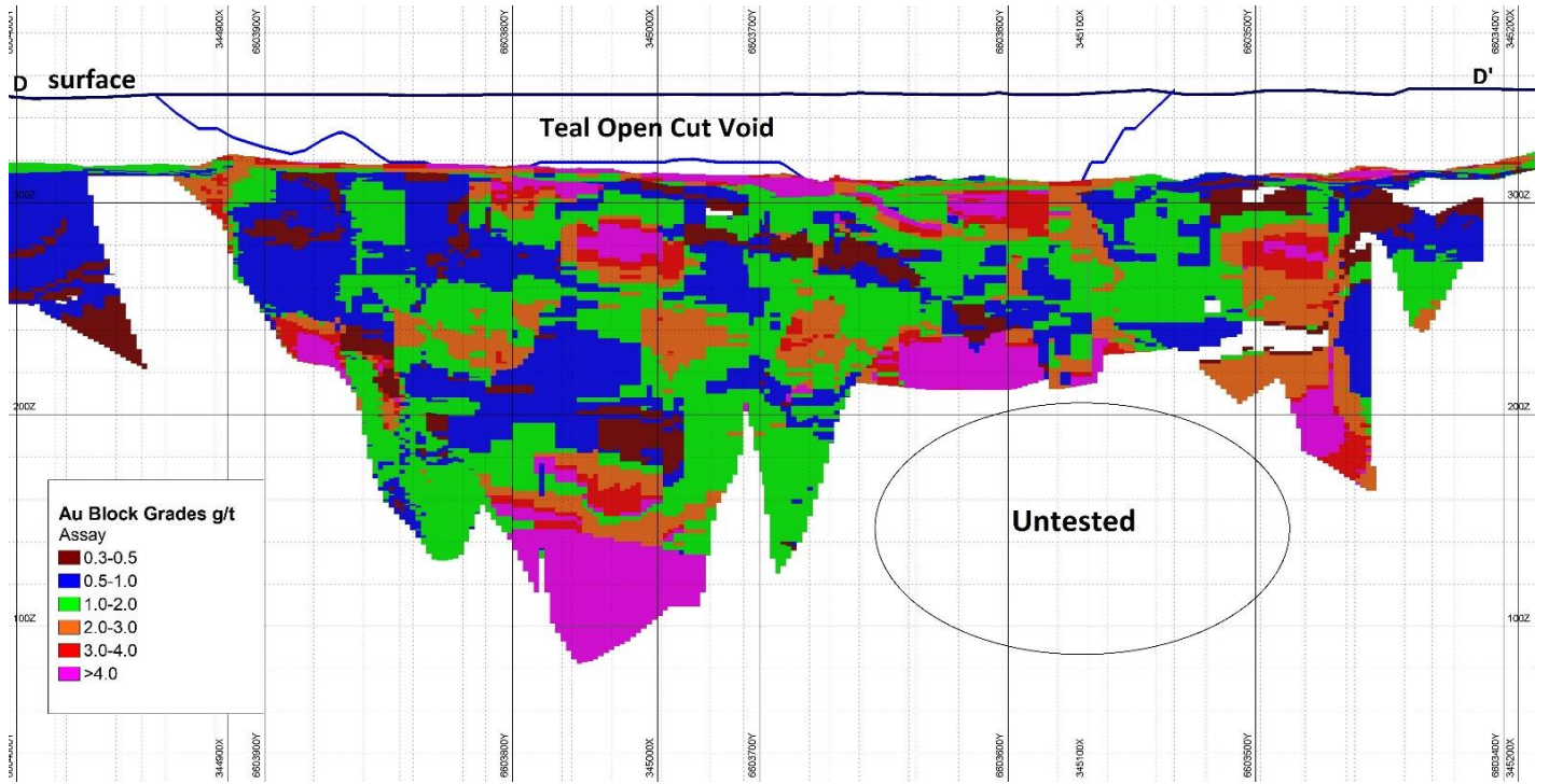
Figure 5: Long section DD' of Teal Block Model (see Figure 4 for location)
