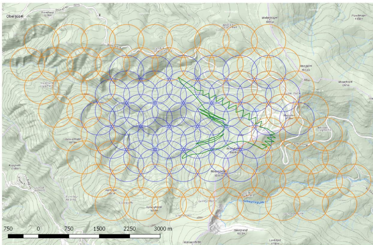
Figure 5; Exploration licences held by European Lithium Limited (blue), new Austrian Lithium Exploration Licences (orange), Amphibolite outline (green).
