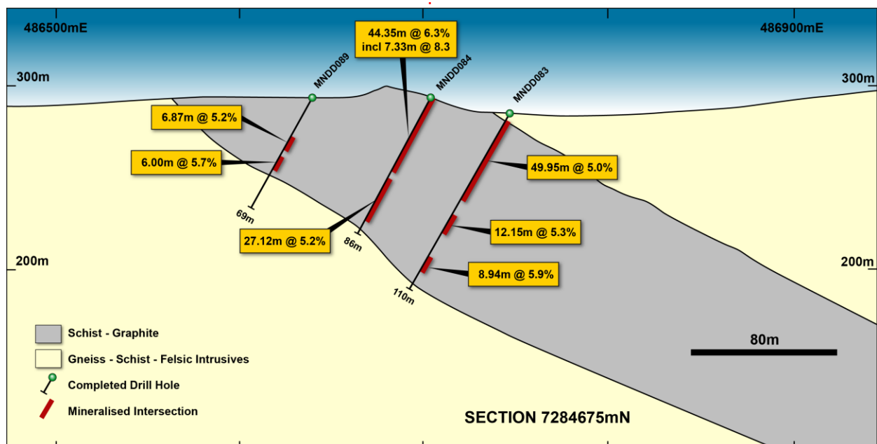
Figure 2 – Haja - Cross Section – 7284675 – (see Figure 1)
