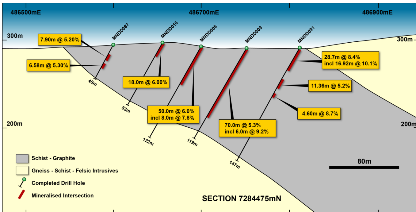
Figure 4 – Haja – Cross Section - 7284475 – (see Figure 1)
