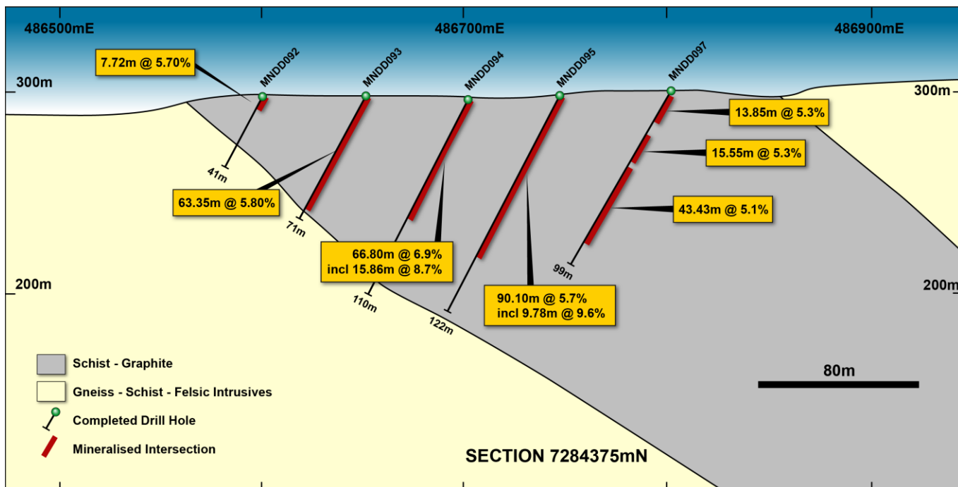
Figure 5 – Haja – Cross Section - 7284375 – (see Figure 1)
