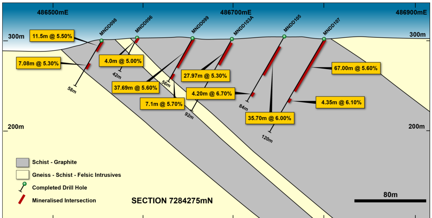
Figure 6 – Haja – Cross Section - 7284275 – (see Figure 1)
