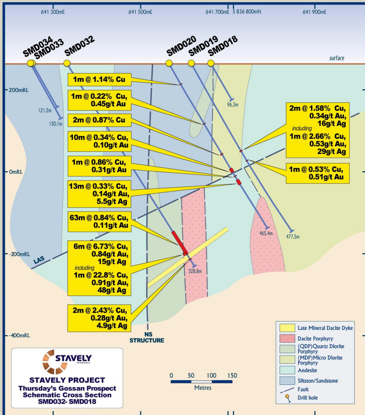
Figure 4. SMD032 Cross-section.
