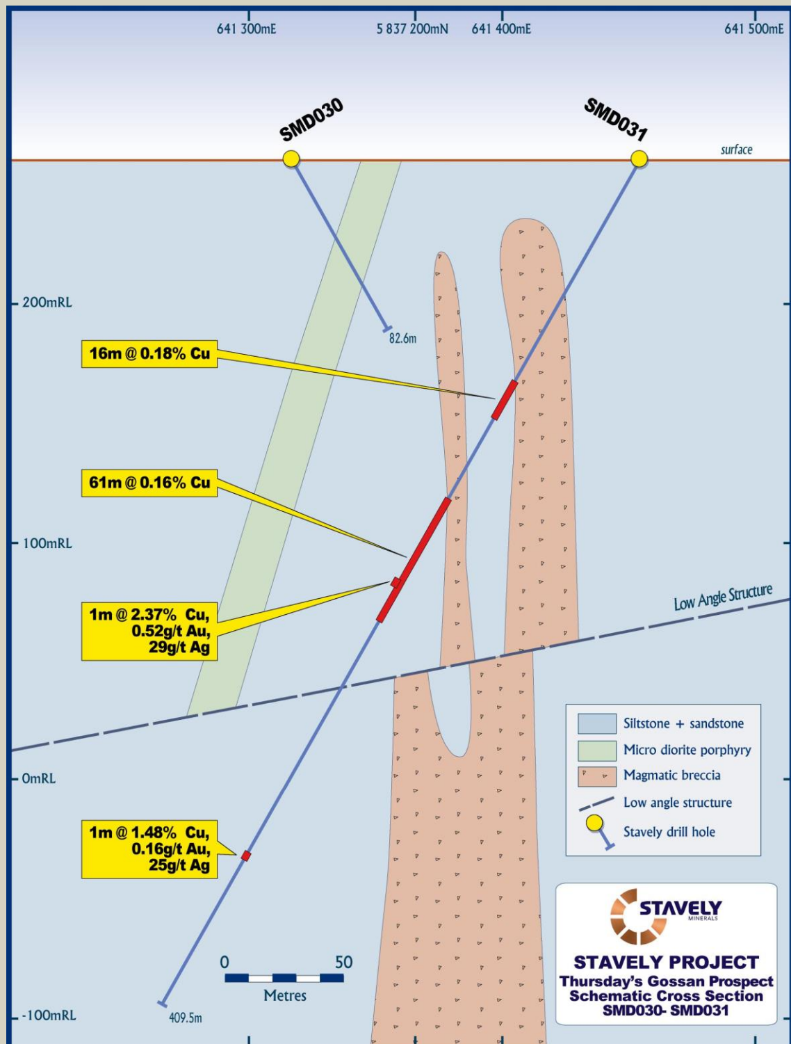
Figure 5. SMD031 Cross-section.
