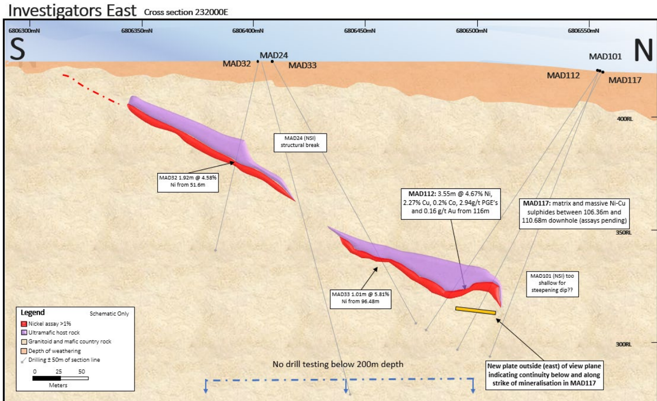
Figure 3 – schematic cross section of the MAD112 Line (facing west) at Investigators based on interpretation of drill hole data. The mineralised ultramafic is open to the north with conductor MAD117:X1 located down plunge of the high-grade mineralisation intersected by MAD112 and MAD117.
