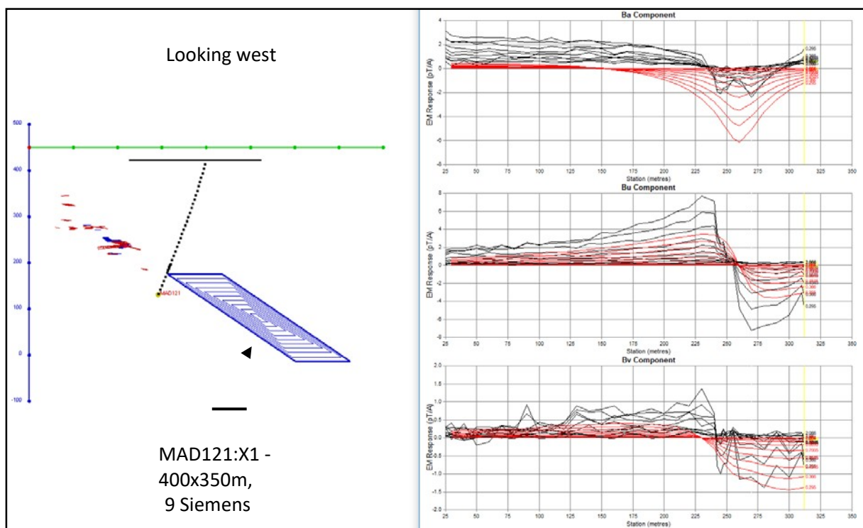
Figure 5 – On left: MAD121 DHEM data results in a large modelled plate. On right: early time (0.3ms to 2ms) linear profiles - red profiles are modelled and black profiles are observed. The sharp negative to positive cross-overs on the radial component (Bu, Bv) indicate a proximal off-hole conductor.
