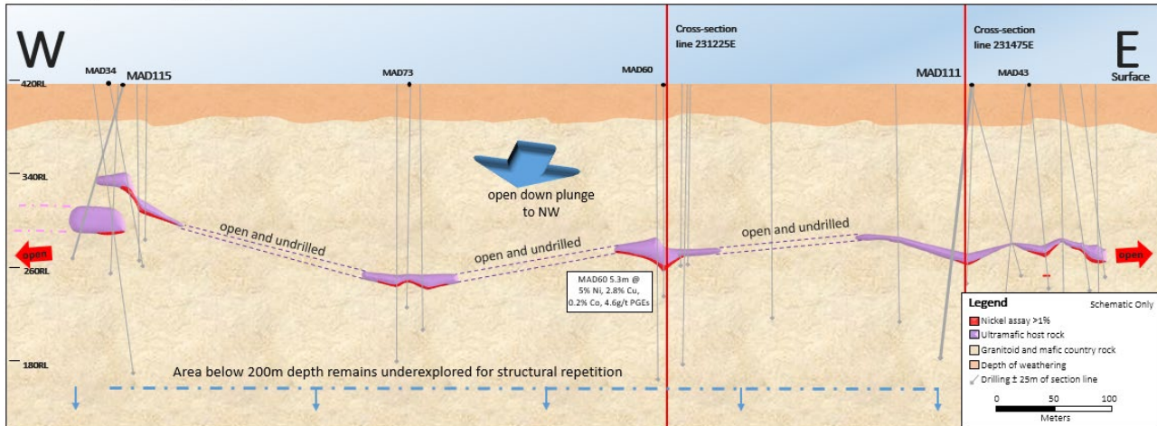
Figure 2 – schematic long section of the Investigators Prospect (facing north) based on interpretation from drill hole data. The MAD60 Line and MAD111 Line are shown, with the MAD112 Line (not shown) a further 530m to the east of the MAD111 Line. Mineralisation remains open to the north and at depth.
