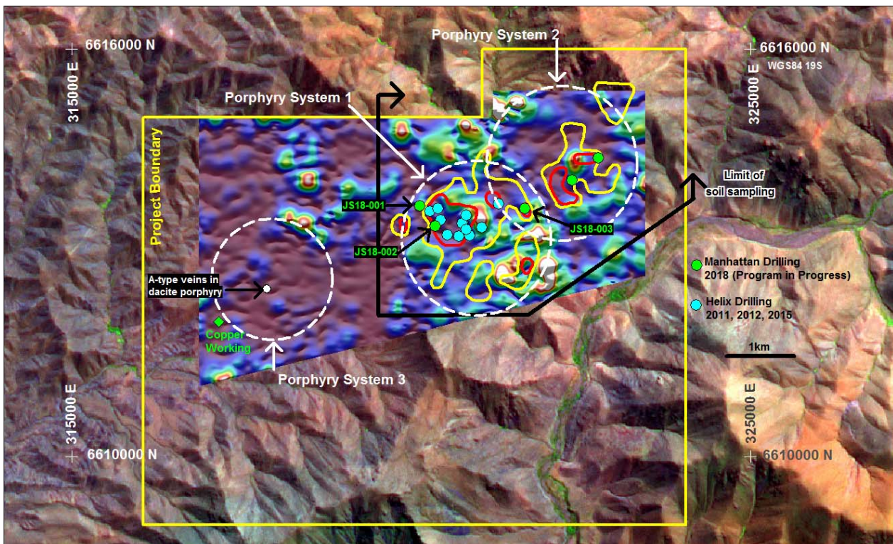
Figure 3 | Imaged aeromagnetic data (analytic signal) showing Helix copper soil anomalies (yellow: +150ppm Cu, red: +500ppm Cu, refer Table 1 for survey details), location of historical drill holes (pale blue dots) and Manhattan drill holes (green dots) and the location of the interpreted three porphyry systems within the Joshua Project Area.
