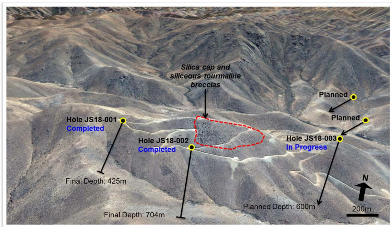
Figure 2 | Relative positions of Manhattan drill holes (completed, in progress and planned) at Joshua shown on north-looking Google image.
