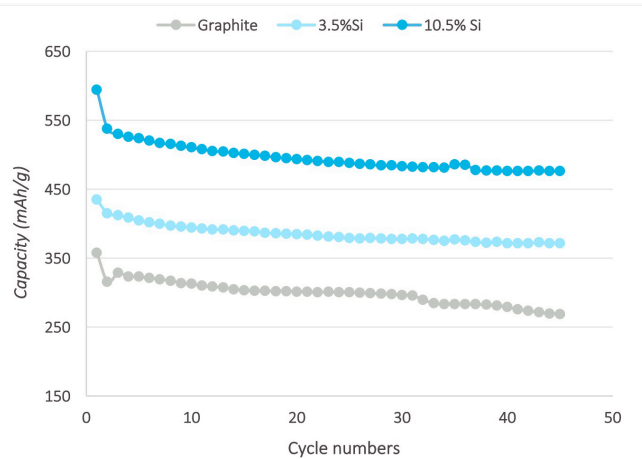
Figure 2 Initial capacity tests of Talnode™-Si versus commercial graphite reference.
