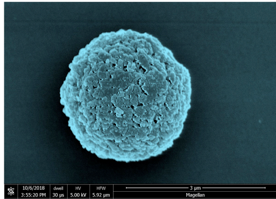
Figure 1 Scanning electron microscope image of Talnode™-Si.
