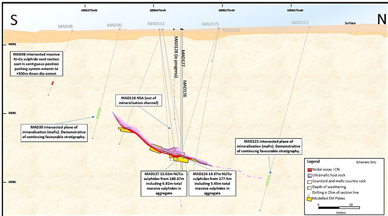
Figure 2 – schematic cross section of the MAD111 Line showing MAD126 and MAD127 and the EM plates modelled on this Line.
