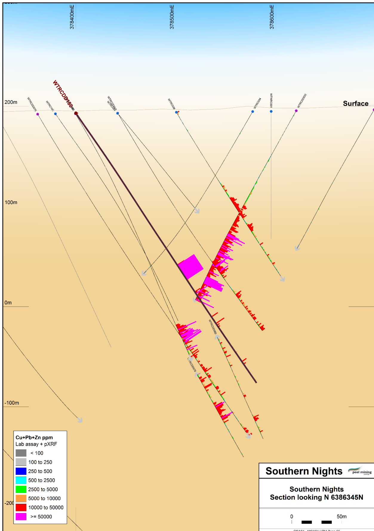
Figure 3: Southern Nights Section 6386345N
