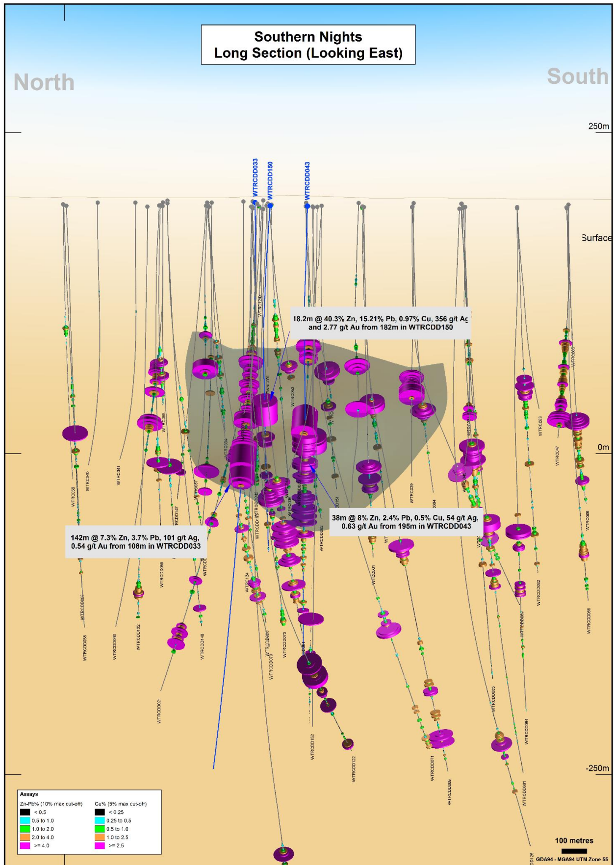
Figure 4: Southern Nights Long Section
