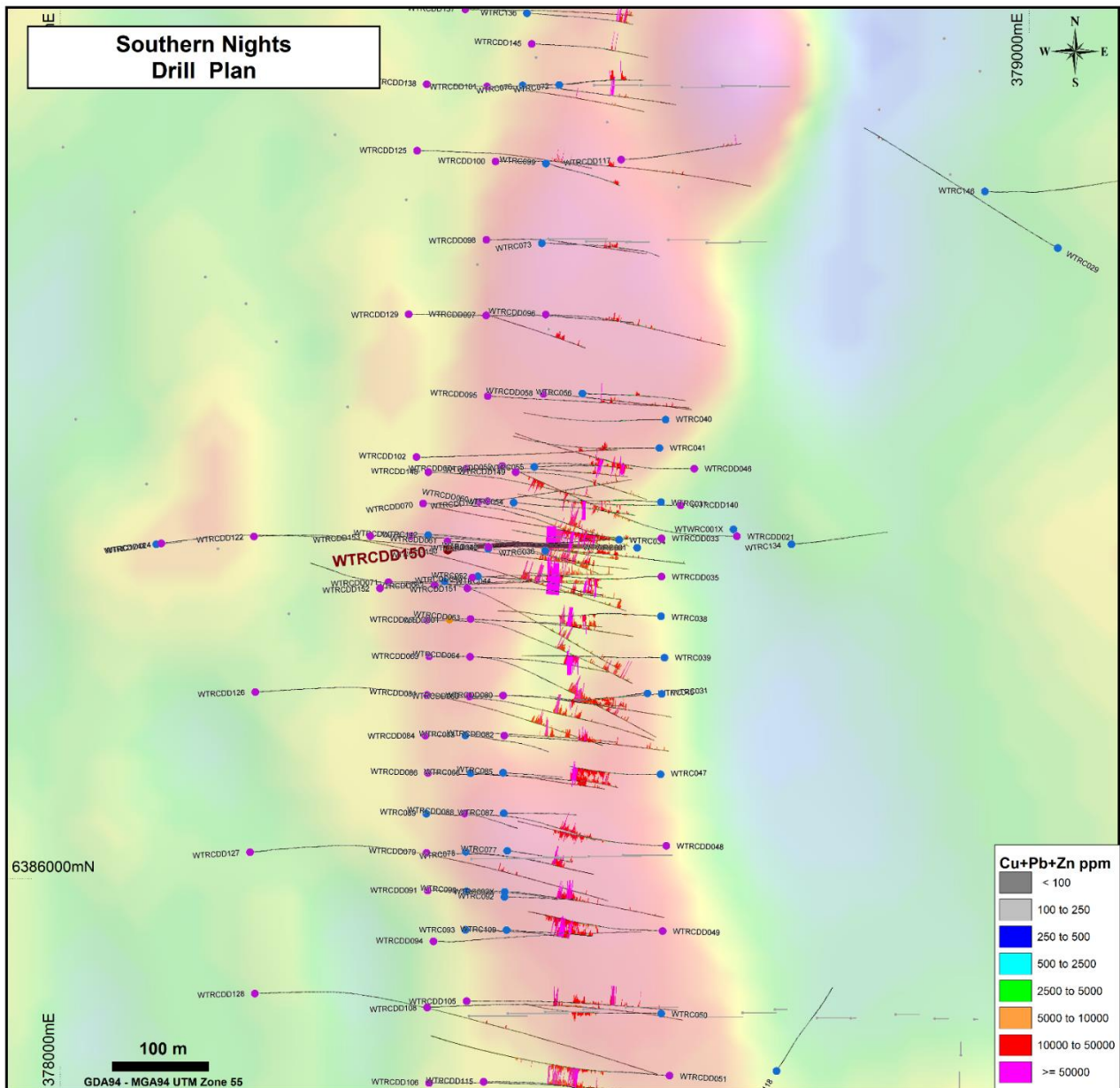
Figure 2: Southern Nights Drill Plan
