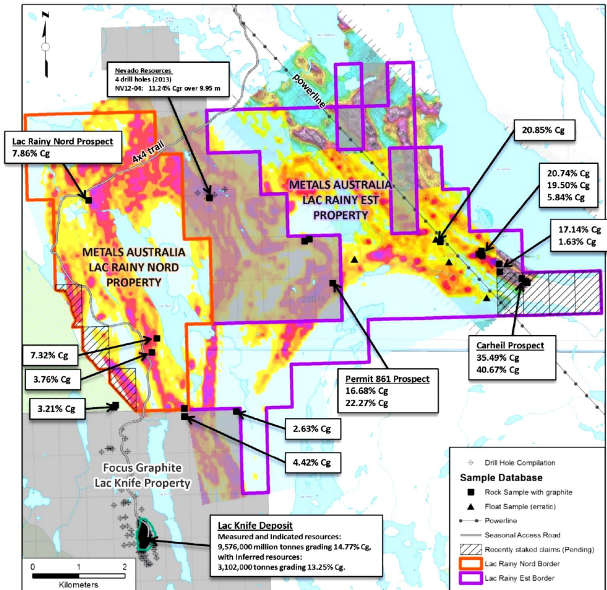
Figure 2: Claim boundaries for the Lac Rainy Nord and Lac Rainy Est Graphite Project overlaid with the results of the recent airborne MAG and TDEM geophysical program
