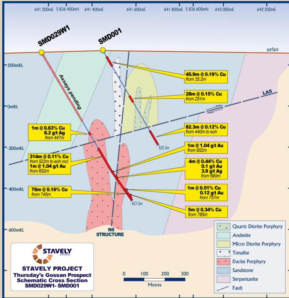
Figure 5. SMD029W1 Cross-section.
