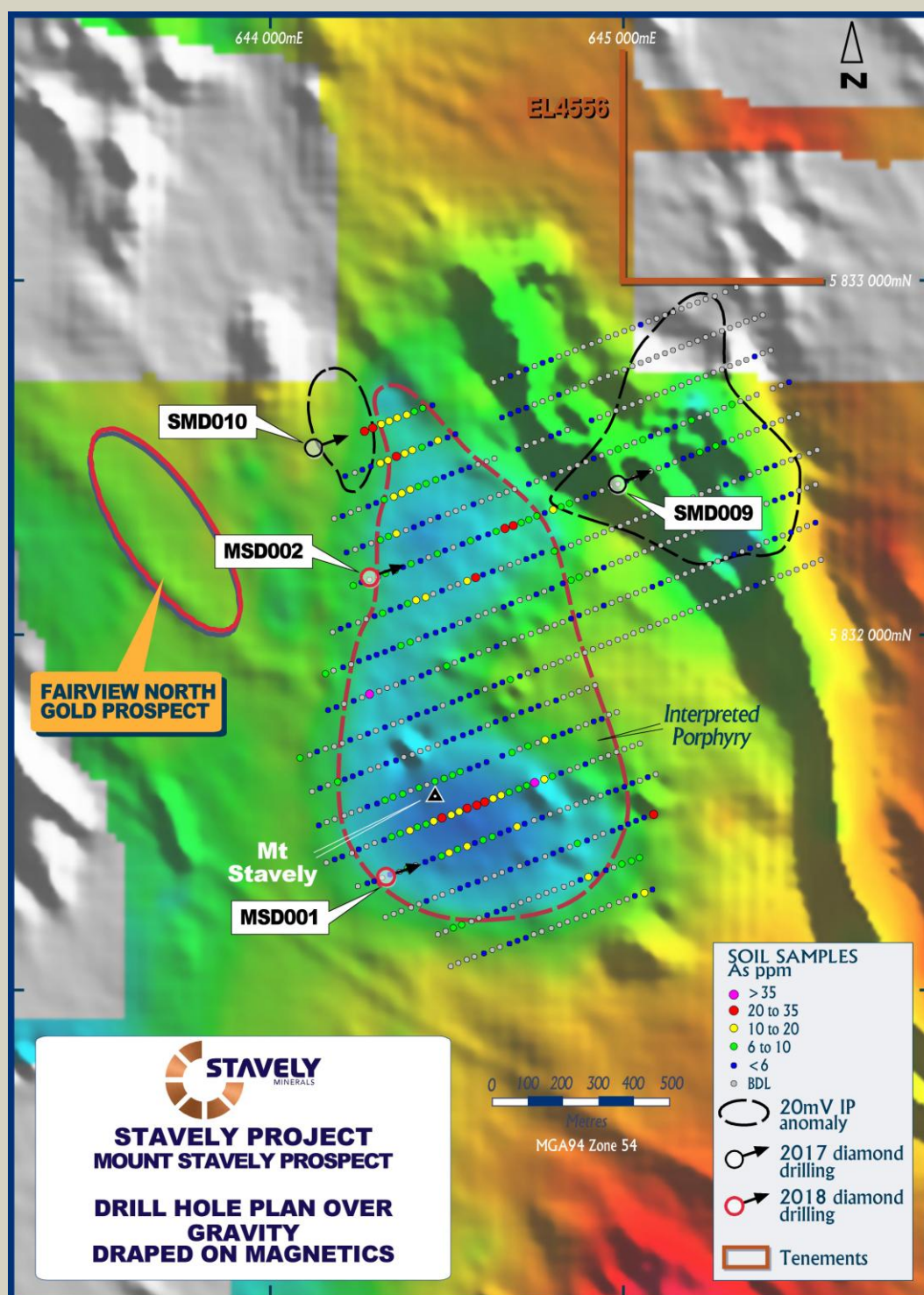
Figure 8. MSD001 and MSD002 drill-hole location plan with grey-scale magnetics overlaid with a colour gravity drape and soil sample arsenic values.
