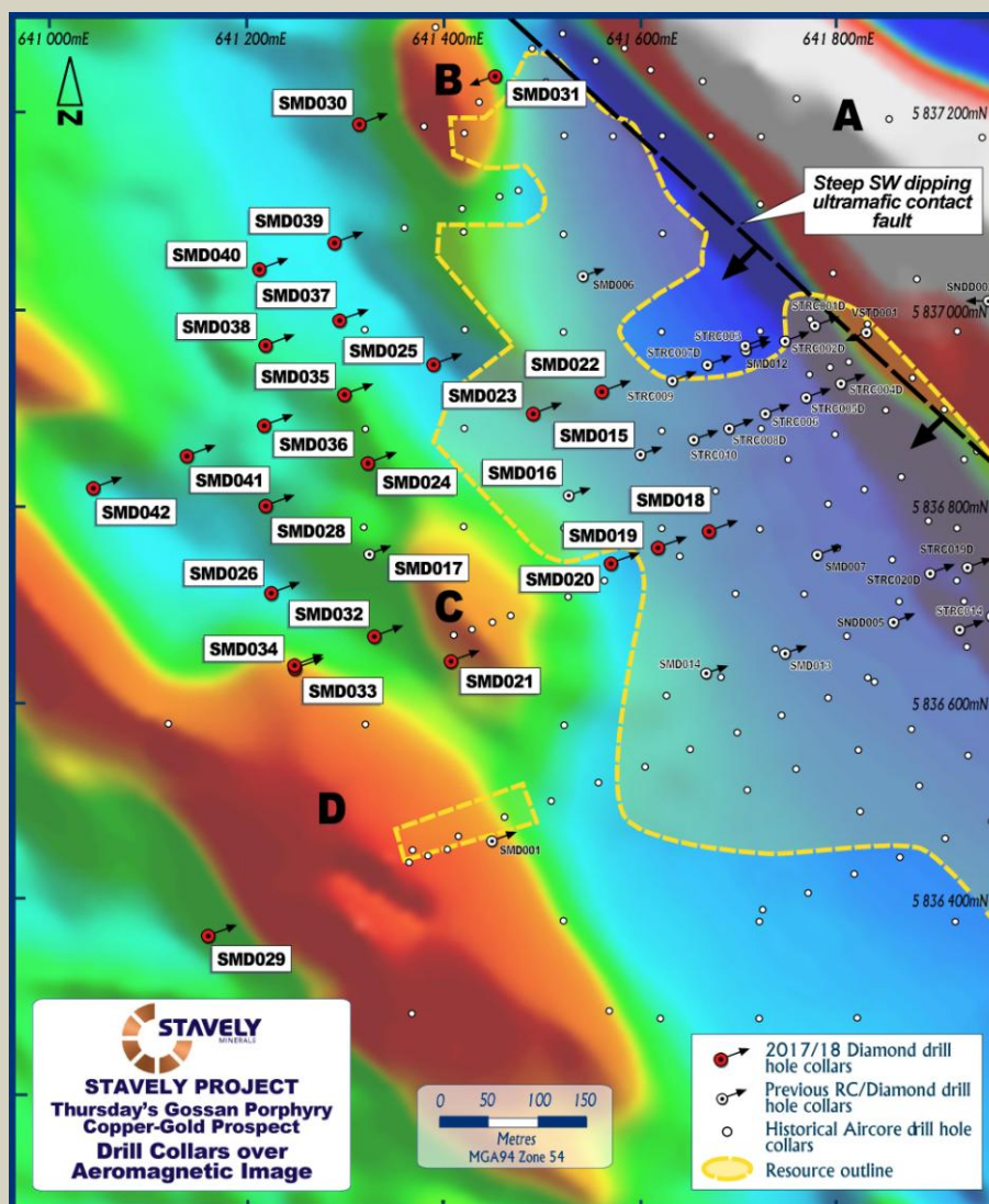
Figure 3. 1VD magnetic image of the area of interest at Thursday's Gossan with drill collars overlaid. All holes drilled at -60 degrees to 070 azimuth with the exception of SMD031. Magnetic features of note annotated A to D.
