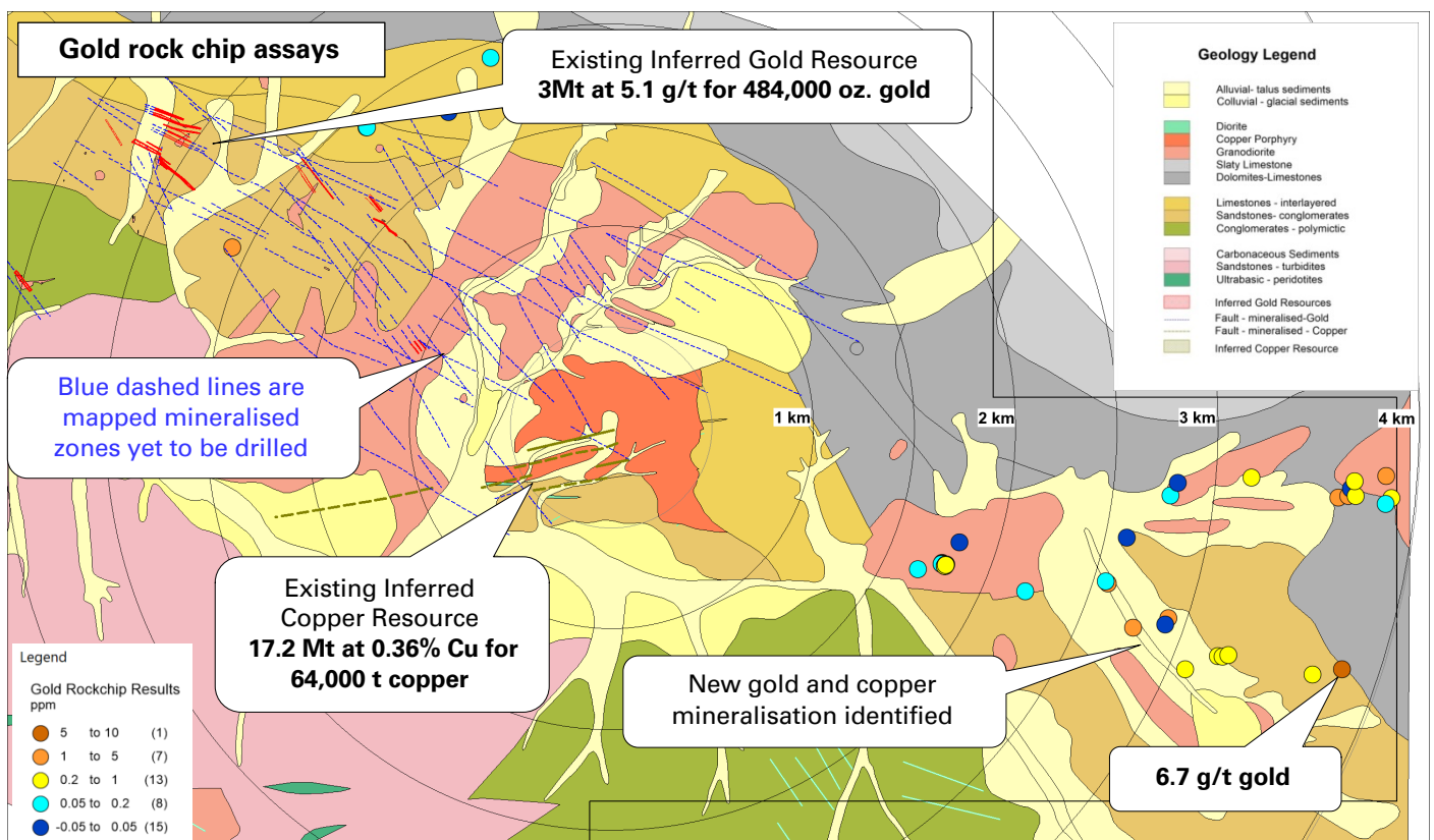
Figure 1: Rock geochemistry (gold) highlights new mineralised zones identified east of the Aucu gold deposit and hints at additional mineralised porphyry intrusions.
