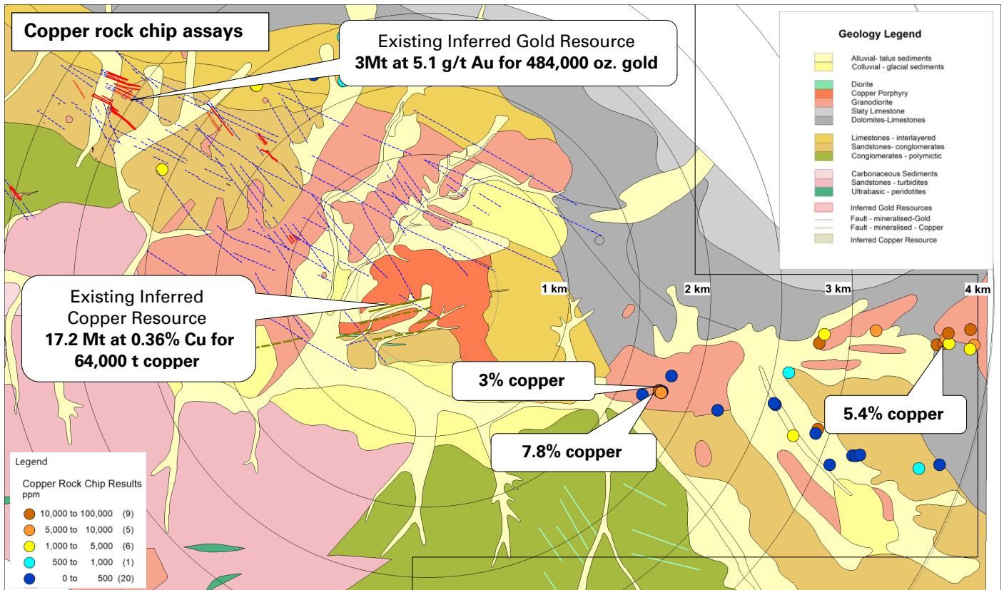
Figure 2: Rock geochemistry (Copper) highlights new mineralised zones identified east of the Aucu gold deposit and hints at additional mineralised porphyry intrusions.
