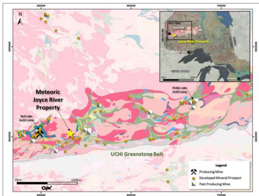
Figure 1: Joyce River Co-Cu-Au Project Location - Regional Geology and Structure
