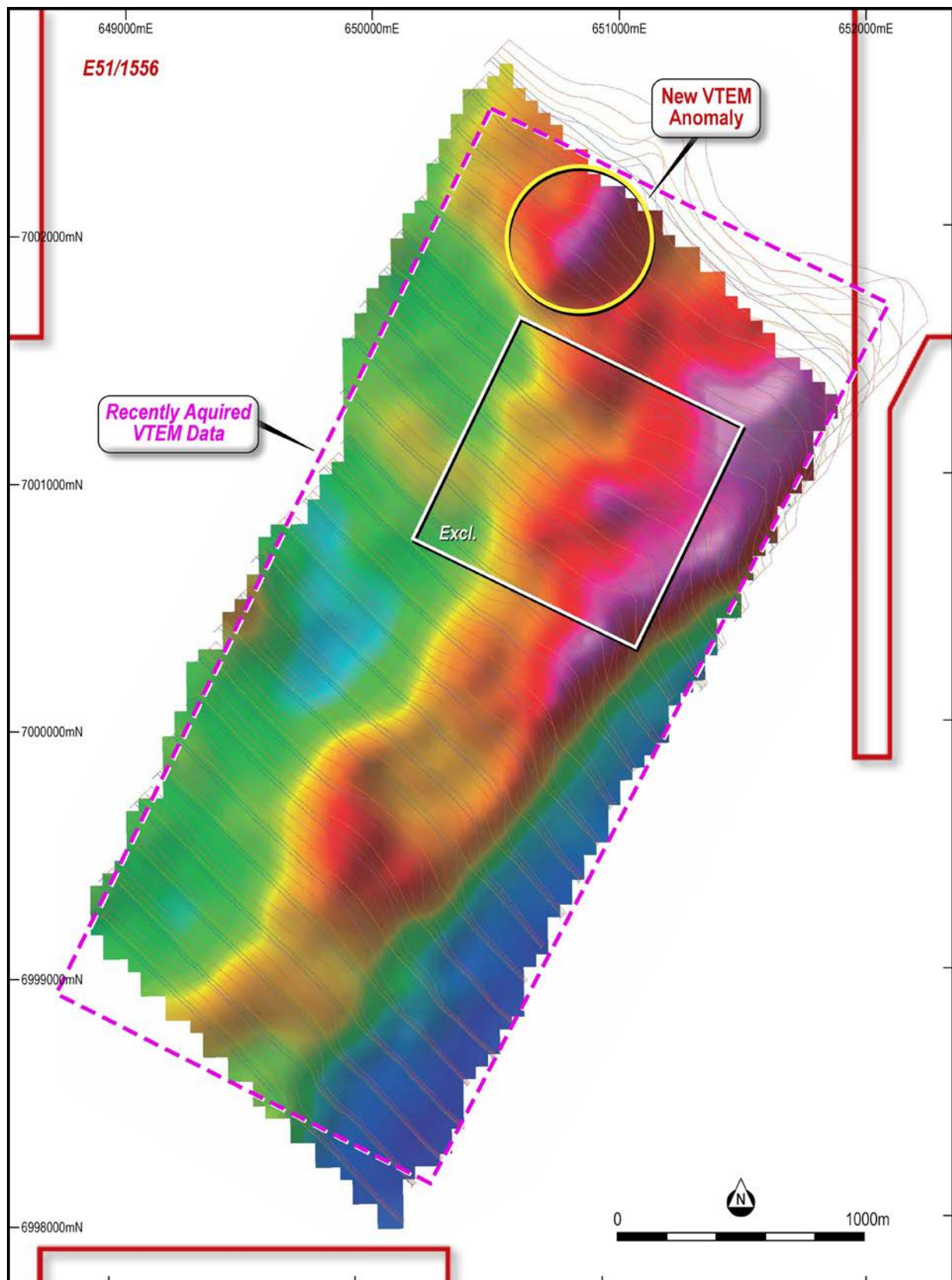
Shallow Conductor in Airborne VTEM (Channel 15) from recently acquired VTEM data.
