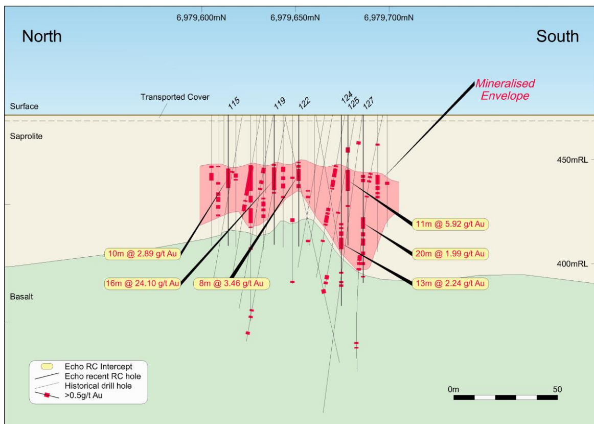
Figure 4: Adder Long-Section
