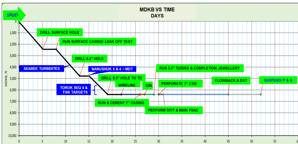
Figure 1 | Winx-1 base case drilling and testing schedule
