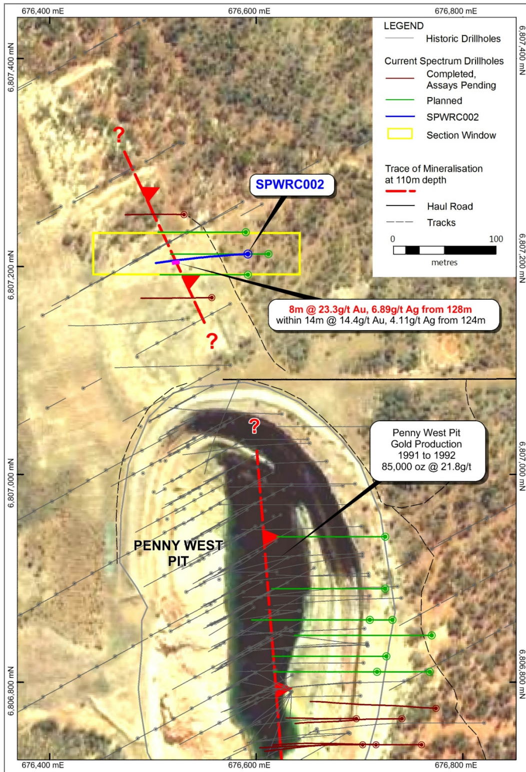
Figure 2. Drill hole location plan with interpretation of Penny West lode and Penny North
