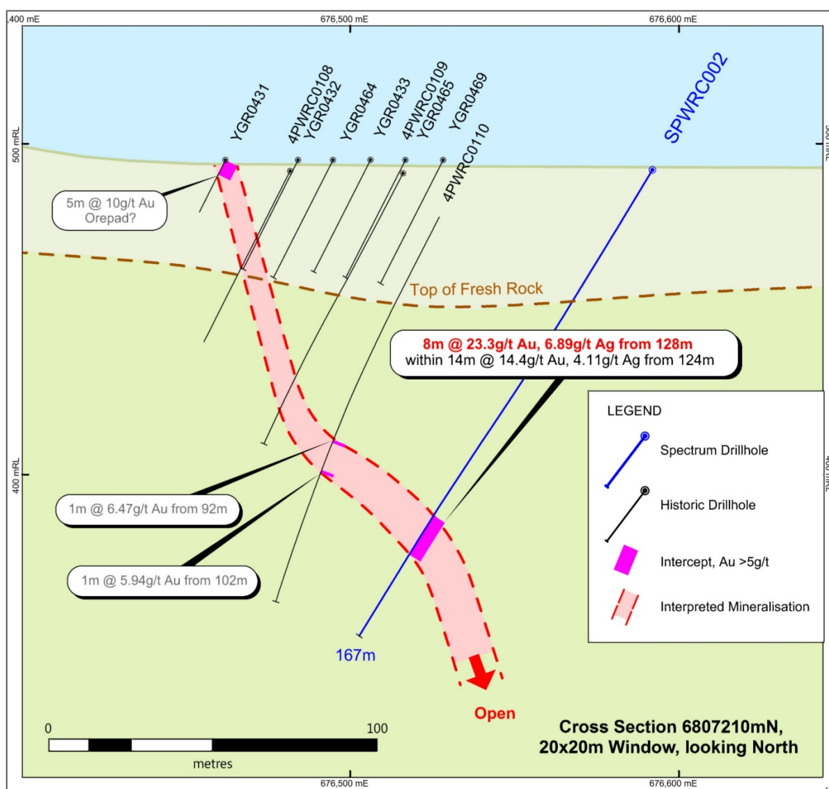
Figure 3. Interpreted cross section showing position of SPWRC002
