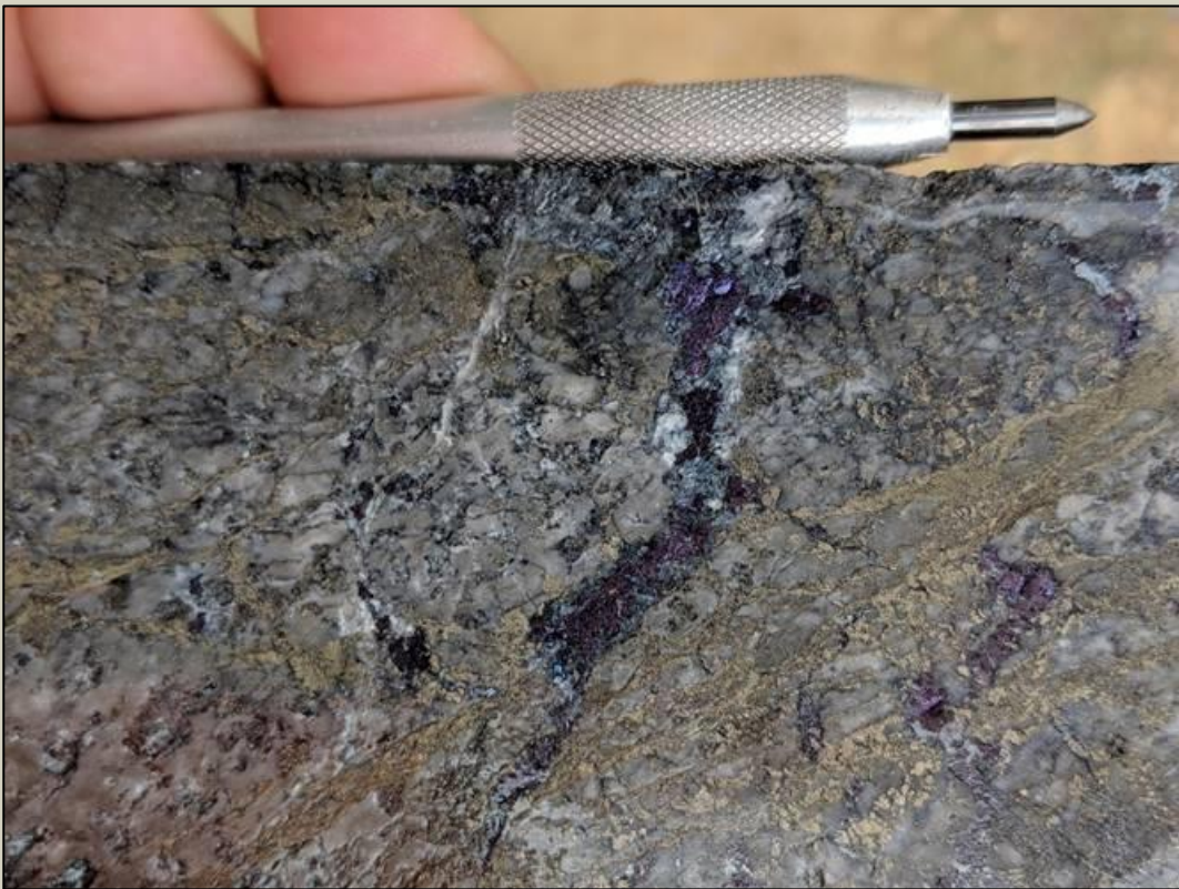
Photo 3. Late bornite-chalcocite cutting earlier pyrite dominant porphyry D veins from 924.2m in SMD044.
