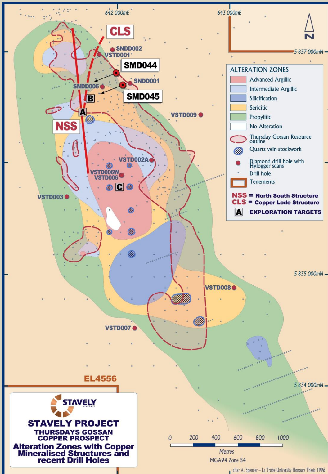
Figure 11. Alteration zonation from the early-phase Victor porphyry(s) showing recent / planned drill holes, the North-South Structure, the Copper Lode Splay Structure and exploration targets 'A', 'B' and 'C' (after Spencer, 1996).
