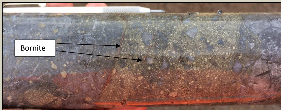
Photo 1. Structural breccia with pyrite clasts and later bornite veining at 580.8m in SMD028.
