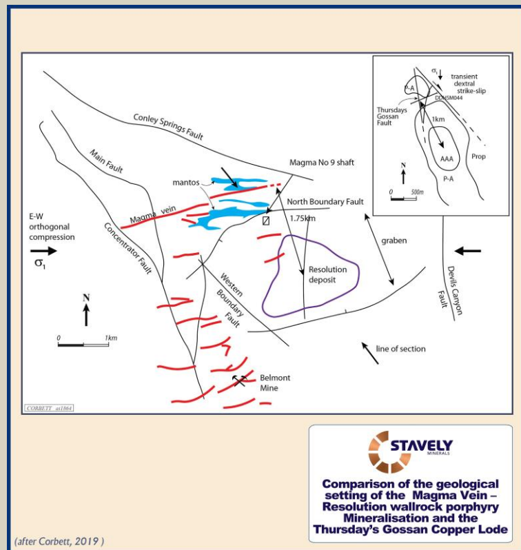
Figure 6. Comparison between the Magma Mine copper lodes / Resolution porphyry and the Thursday's Gossan setting – see Figure 11 for the context of the inset figure.
