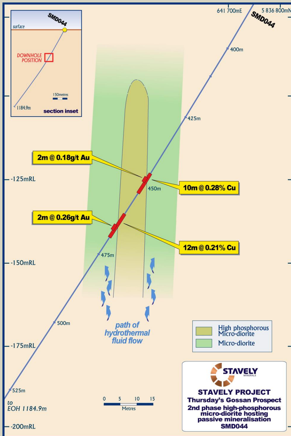
Figure 10. SMD044 showing 'passive' mineralisation on the margins of the phase-2 high-P microdiorite indicating the existence of a phase-3 porphyry responsible for this mineralisation and the high-grade copper lode-style mineralisation.
