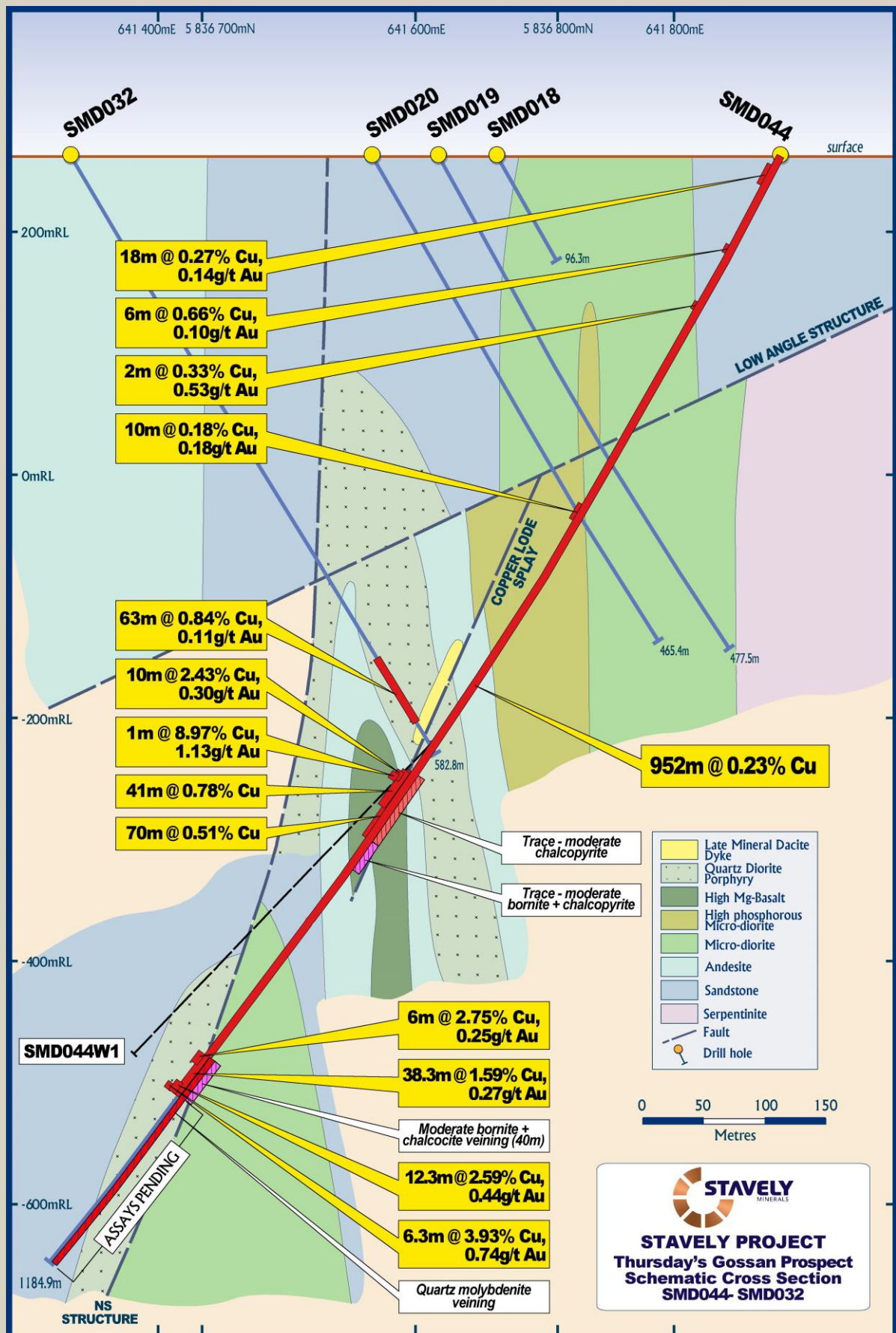
Figure 3. SMD044 Cross-section.
