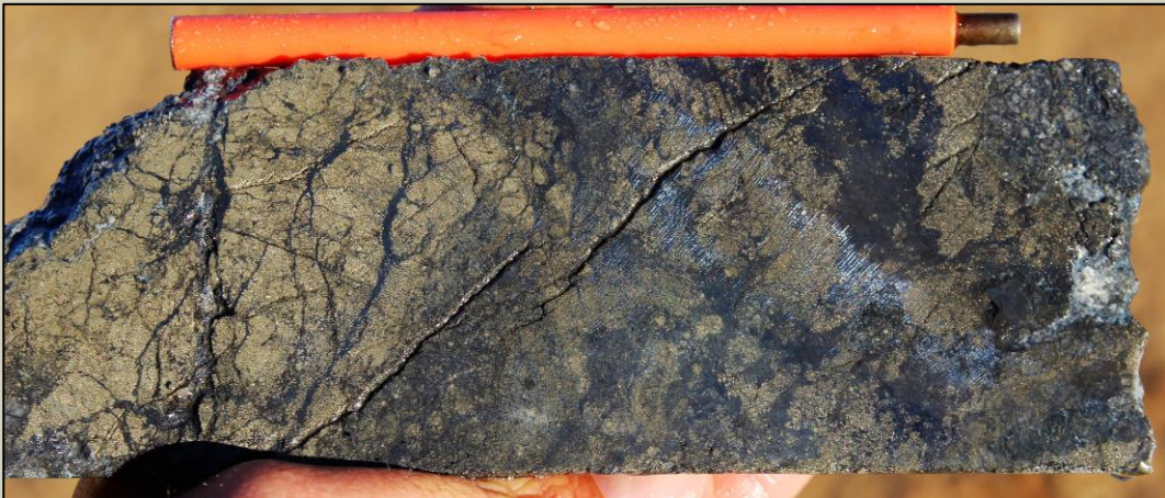
Photo 2. Copper lode-style chalcopyrite-bornite-covellite-chalcocite mineralisation cutting earlier pyrite dominant porphyry D veins in the CLS from 542.5m in SMD032—note the chalcocite occurs as late network veins within the more massive sulphides.
