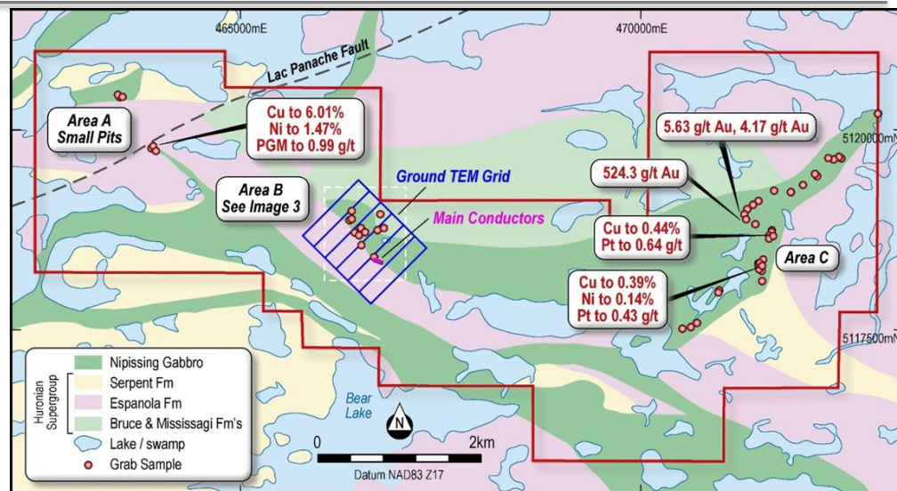
Image – Panache Project – Local Geology with Grab Sampling, Ground TEM Grid and Location of Conductors.
