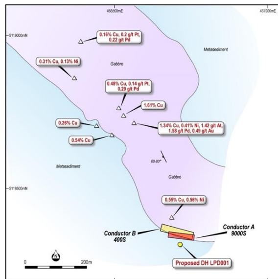
Image – Panache Project –Regional Geology and Target Area Location
