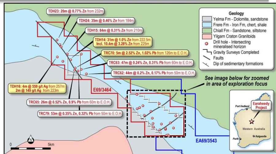
Image: Project Geology, Significant zinc mineralisation over an area of 20km by 3.5km and area of exploration focus
