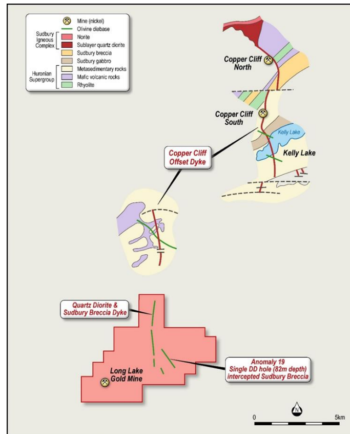
Image – Long Lake Project - Highlighting the Copper Cliff Offset Dyke and the Inferred Sudbury Breccia Dyke
