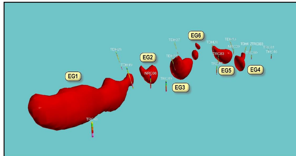
Image: Drill Hole Intercepts with Gravity Targets over TMI Aeromagnetic Plan – Southeast Area.
