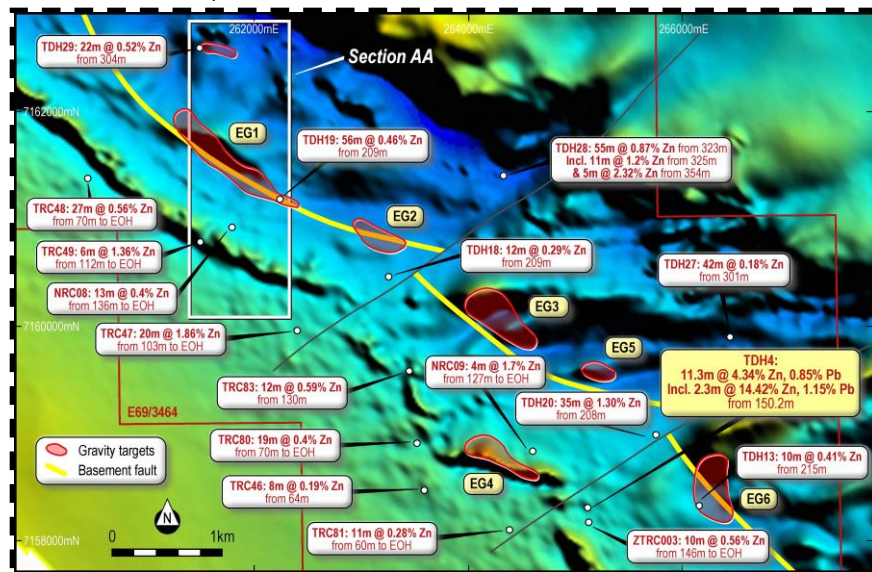
Image: Area of Exploration Focus see top image for location: Drill InterceptsGr and Gravity Drill Targets over TMI Aeromagnetics.
