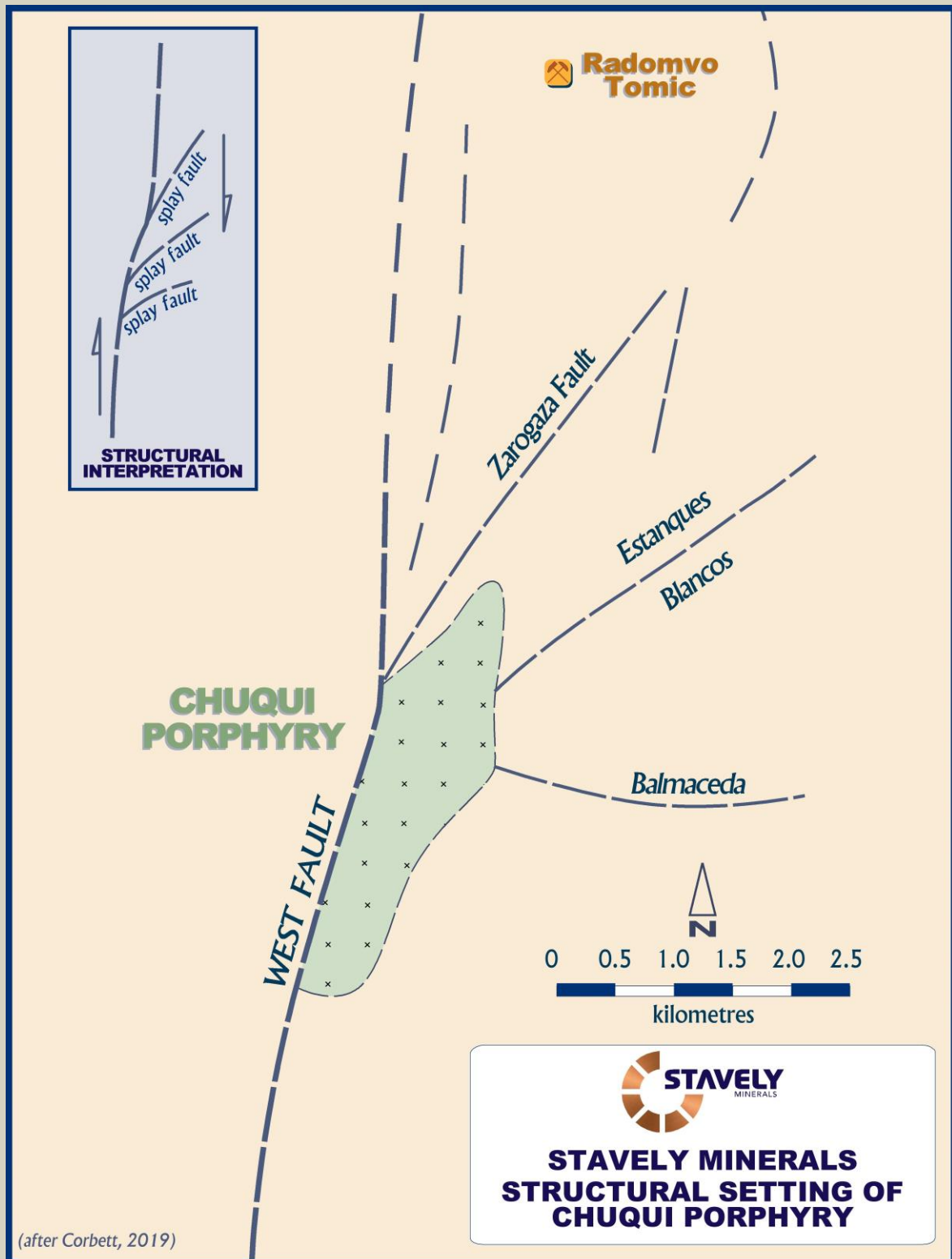
Figure 8. Structural setting of the Chuquicamata porphyry copper deposit. Intrusive phases, alteration and mineralisation are strongly influenced by the interaction between the West Fault and the splay faults.
