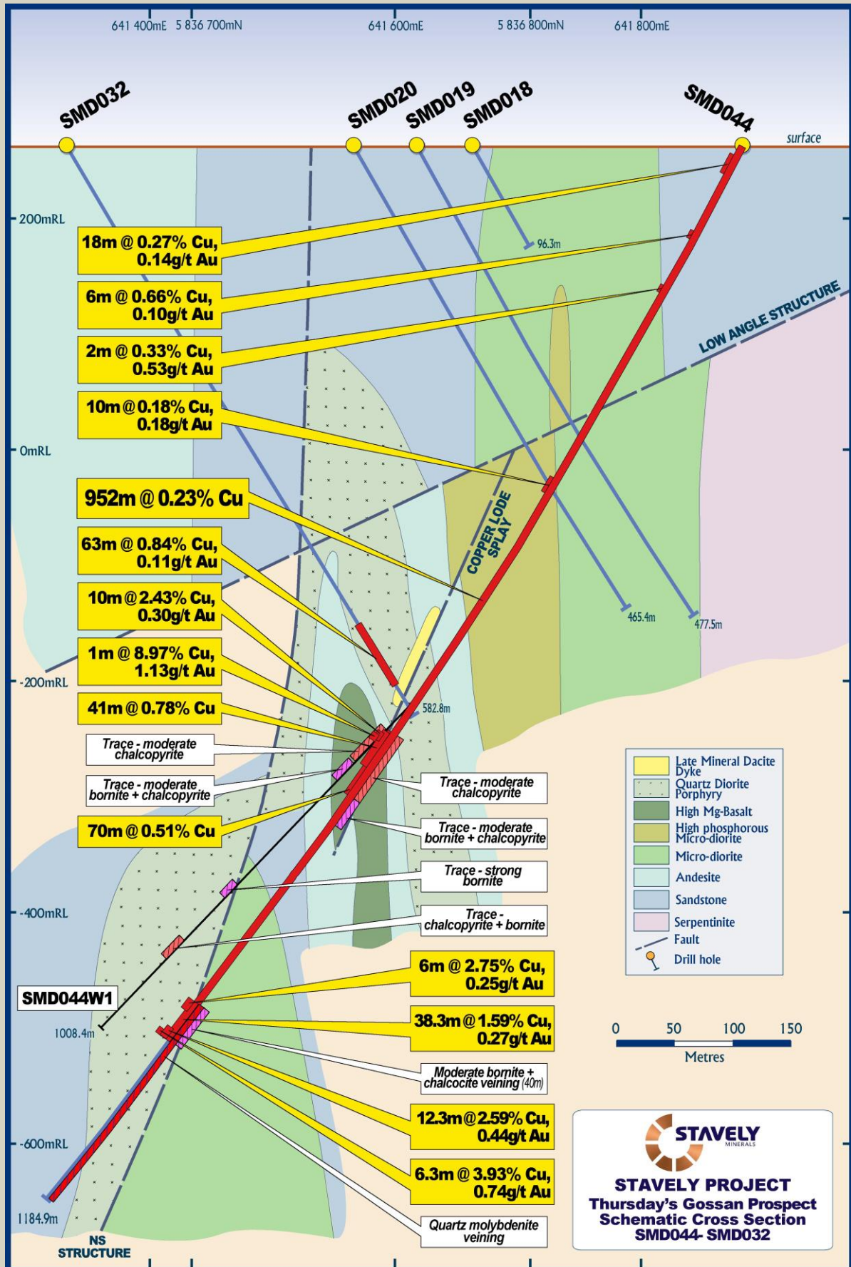
Figure 3. SMD044 Cross-section.
