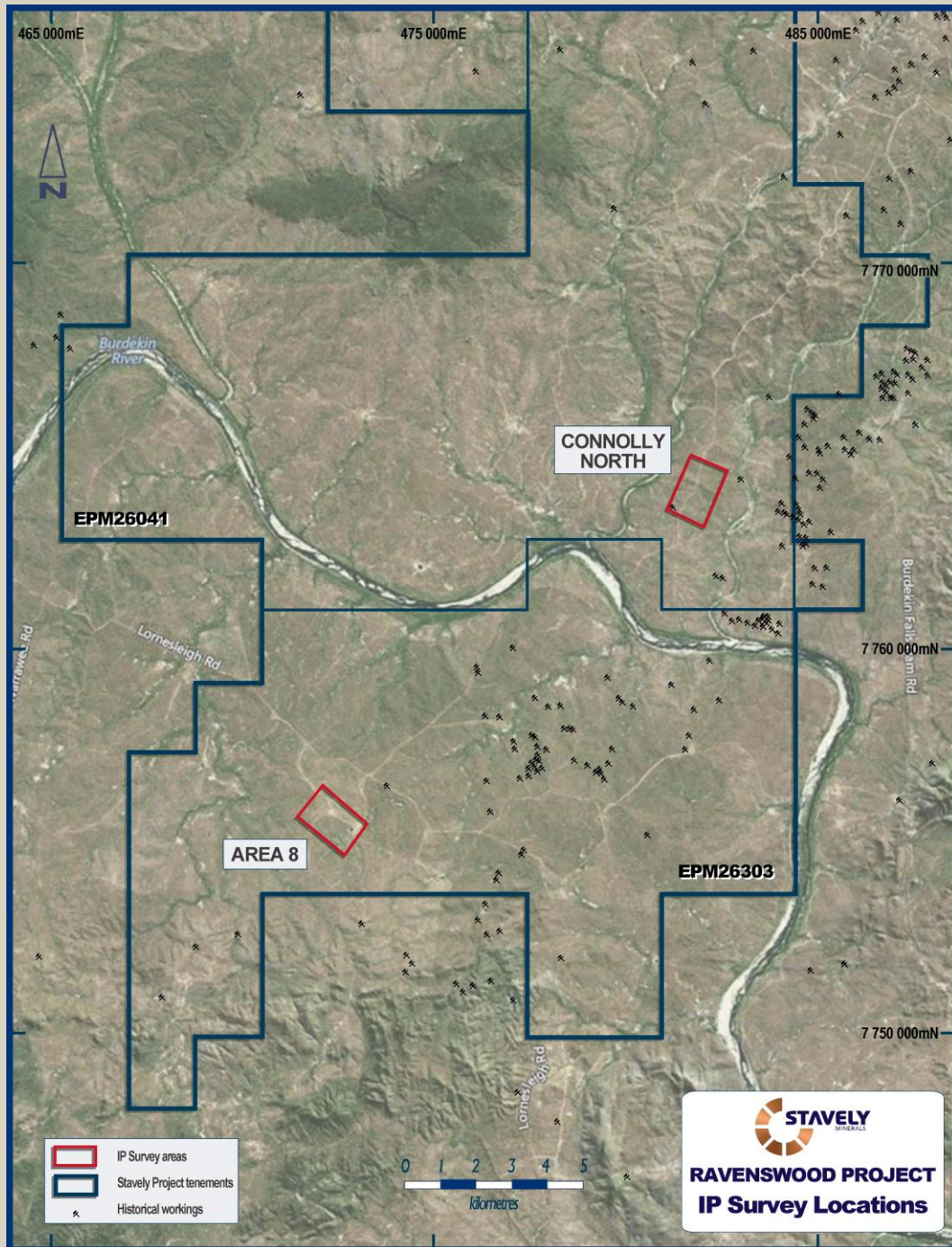
Figure 10. Ravenswood Project – Connolly North and Area 8 location plan.
