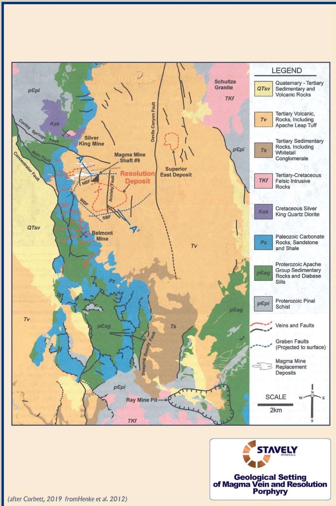
Figure 4. Geology plan of the Magma Copper Lodes and the Resolution porphyry projected to surface.
