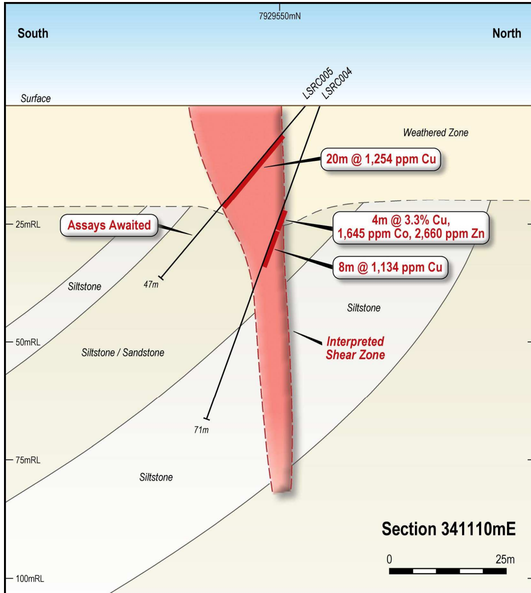
Figure 4: Cross section view of drilling at Lincoln Springs prospect. Section 341110mE.
