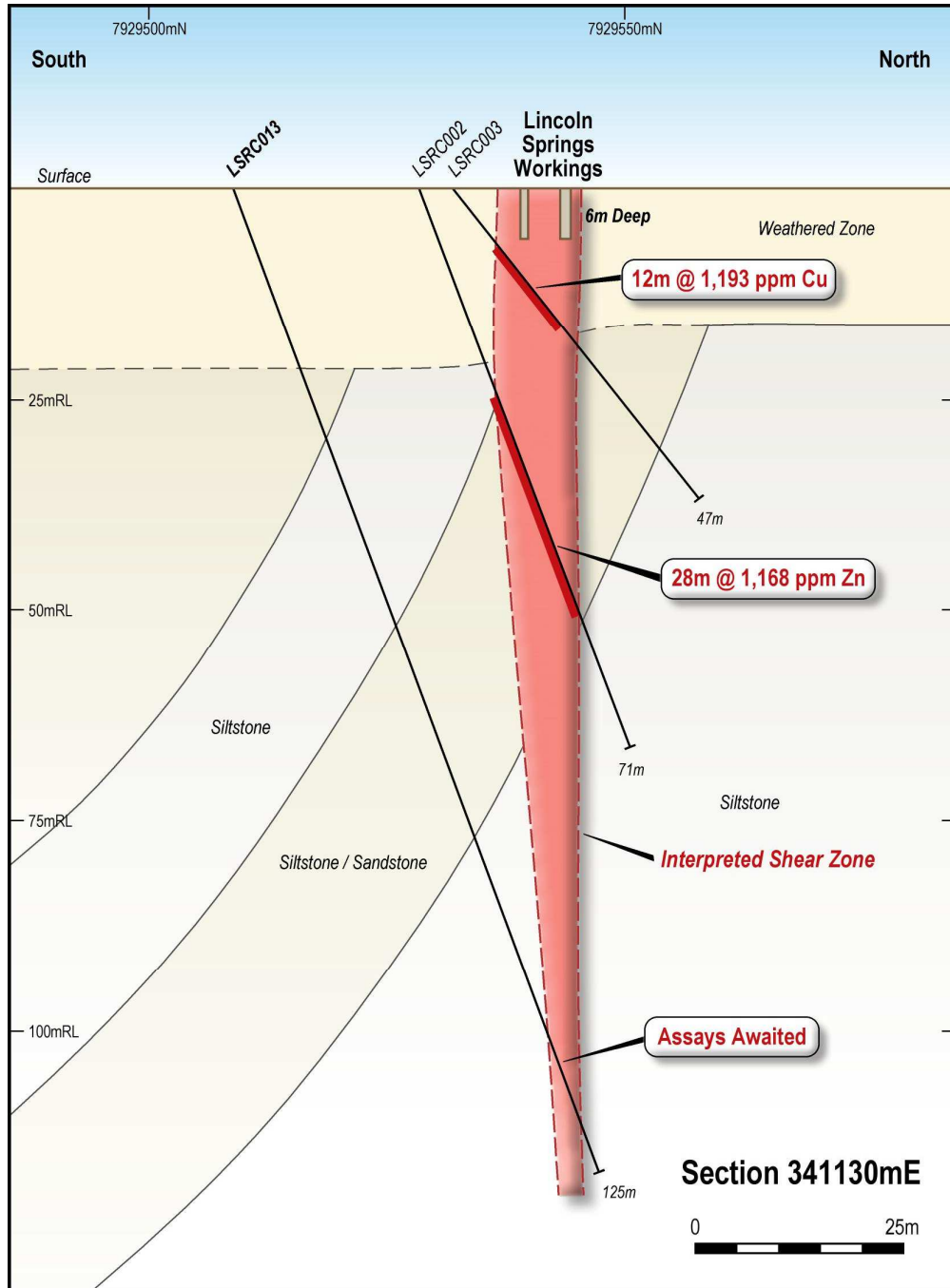
Figure 3: Cross section view of drilling at Lincoln Springs prospect. Section 341130mE.
