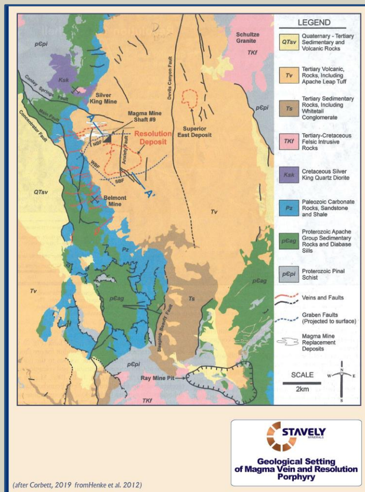
Figure 4. Geology plan of the Magma Copper Lodes and the Resolution porphyry projected to surface.
