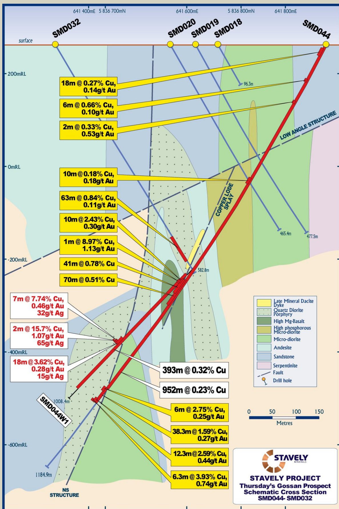
Figure 3. SMD044 Cross-section.
