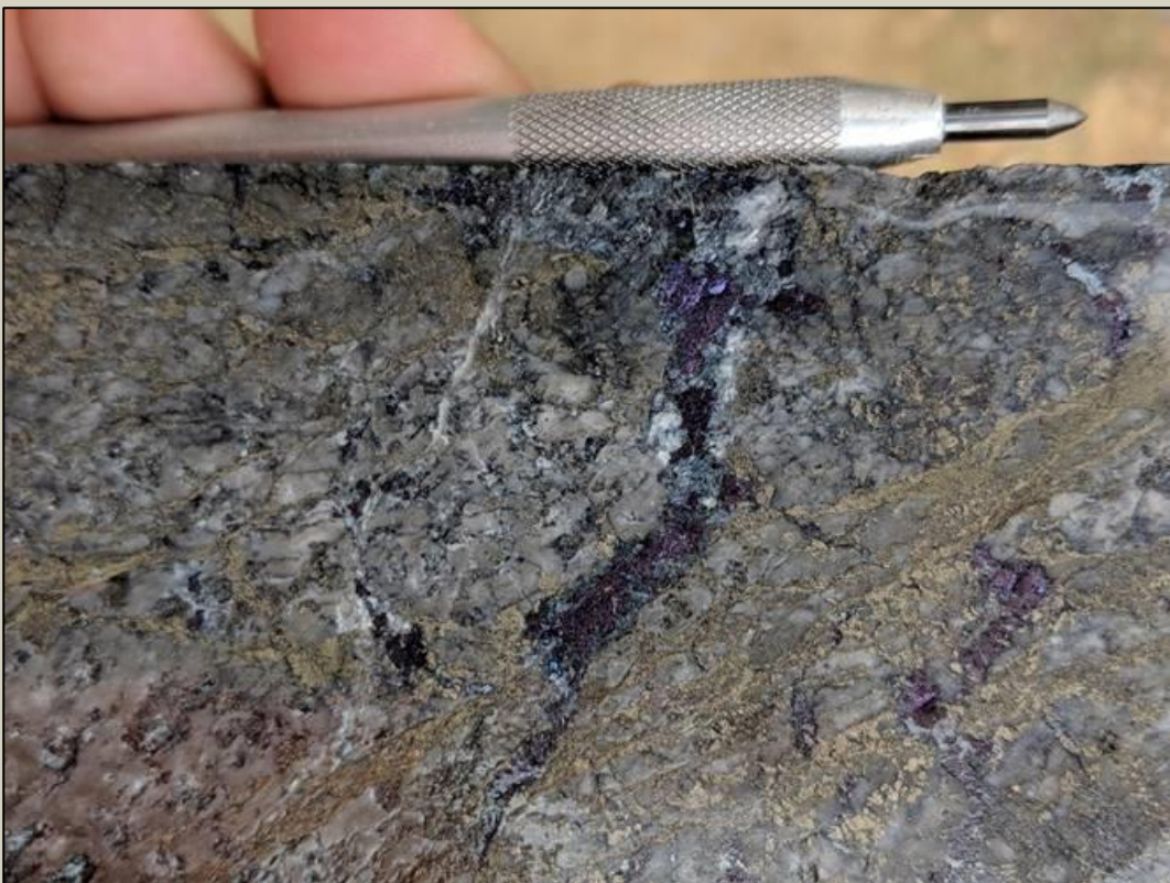
Photo 5. Late bornite-chalcocite cutting earlier pyrite dominant porphyry D veins from 924.2m in SMD044.
