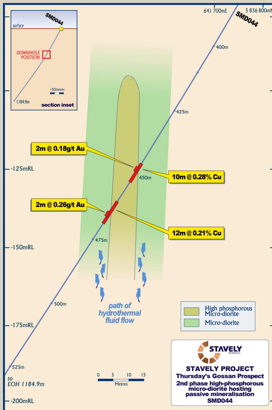
Figure 9. SMD044 showing 'passive' mineralisation on the margins of the phase-2 high-P microdiorite indicating the existence of a phase-3 porphyry responsible for this mineralisation and the high-grade copper lode-style mineralisation.
