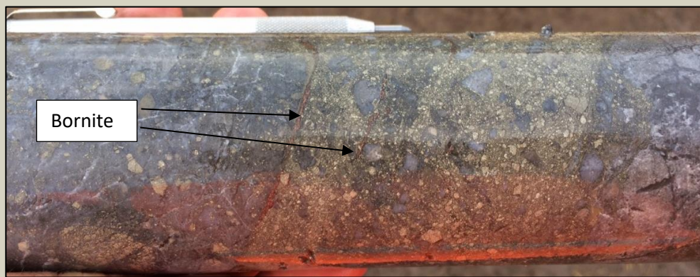
Photo 3. Structural breccia with pyrite clasts and later bornite veining at 580.8m in SMD028.
