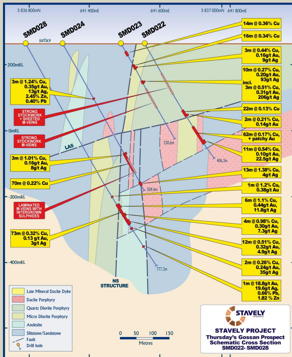
Figure 8. SMD028 Cross-section.
