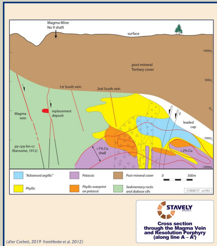
Figure 5. Cross section A-A' from Figure 4 showing the relationship between the Magma Mine copper lodes and the Resolution porphyry copper mineralisation.
