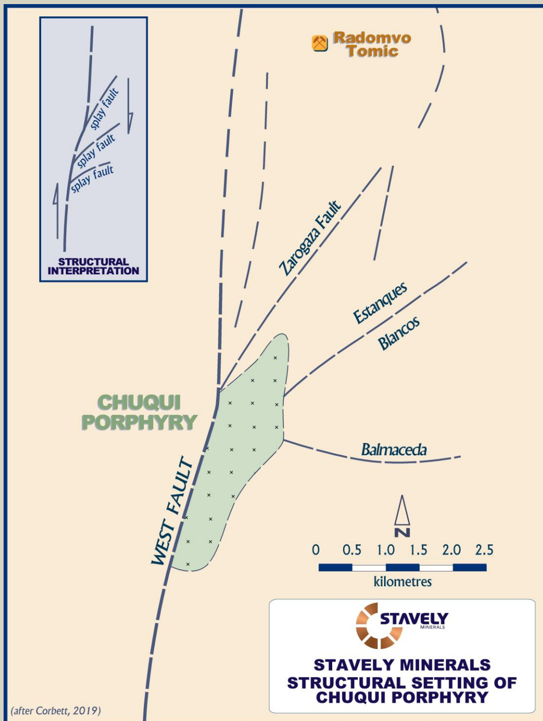
Figure 7. Structural setting of the Chuquicamata porphyry copper deposit. Intrusive phases, alteration and mineralisation are strongly influenced by the interaction between the West Fault and the splay faults.
