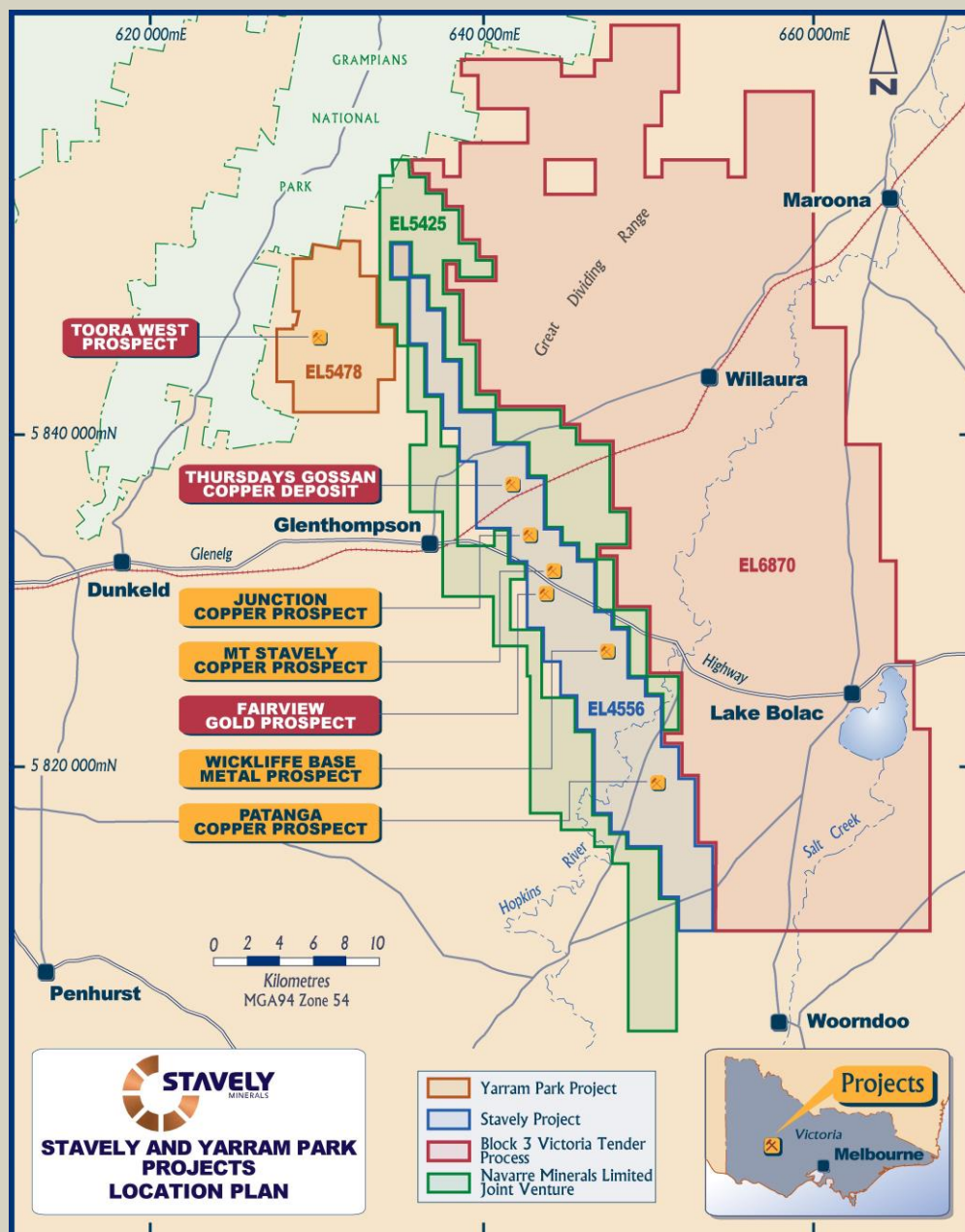
Figure 1. Stavely Project location plan.
