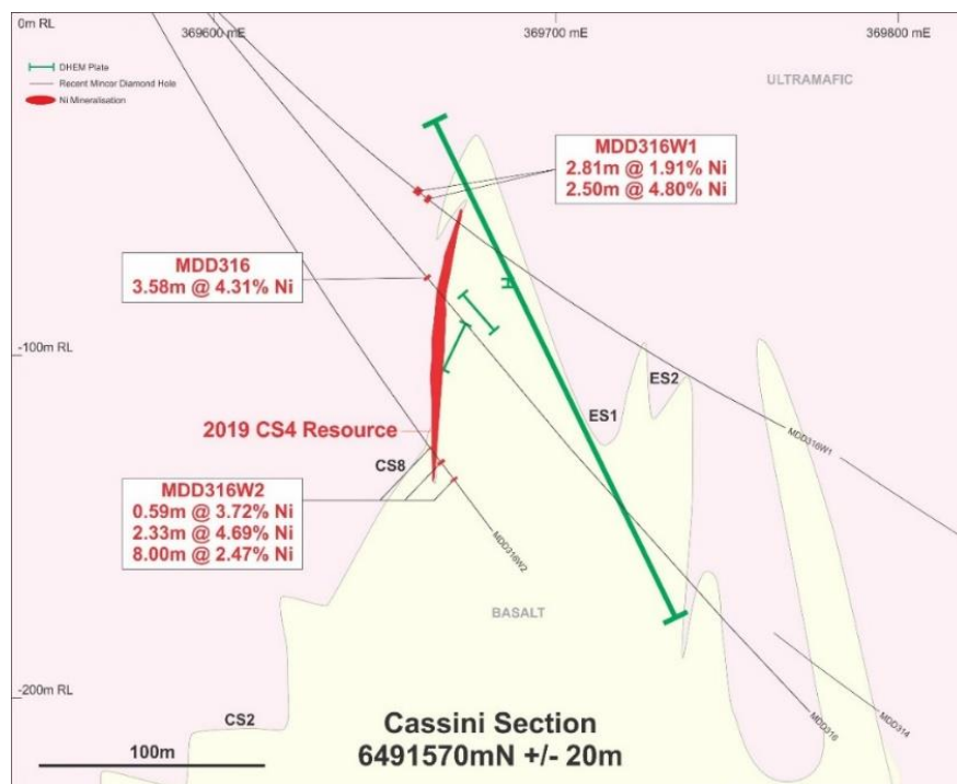
Figure 2: Cassini cross-section 6491570N
