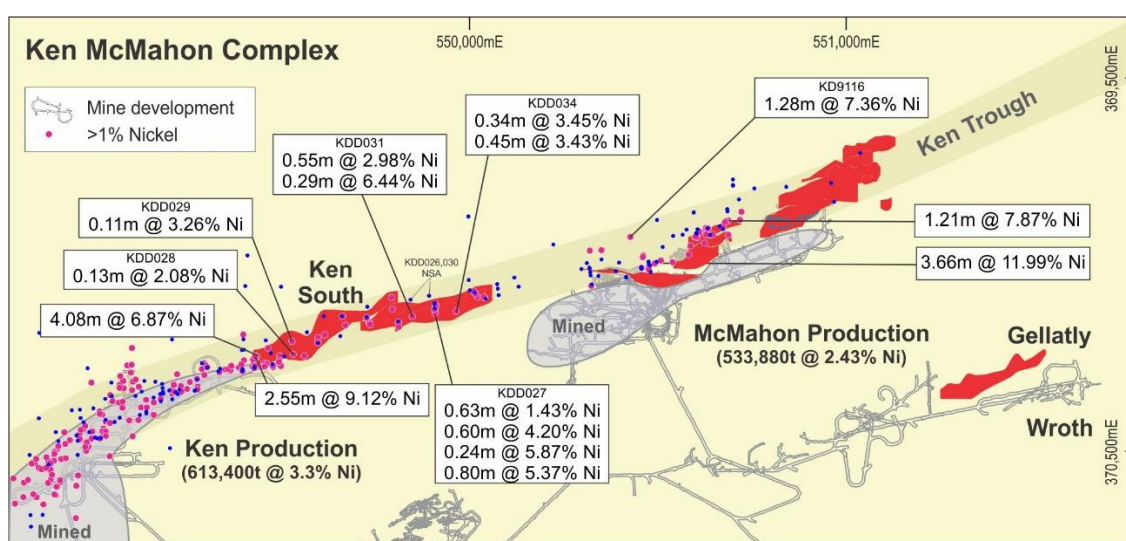
Figure 3: Plan view of the targeted Ken Trough with existing Mineral Resources
