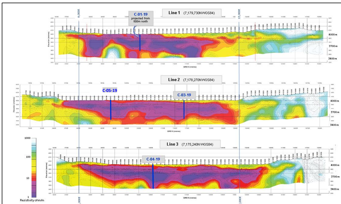
Figure 2: CSAMT Profiles 1-3 - Interpreted model showing lowly resistive brine saturated materials (in purple/blue) with possible dry materials (yellow) & location of drillholes
