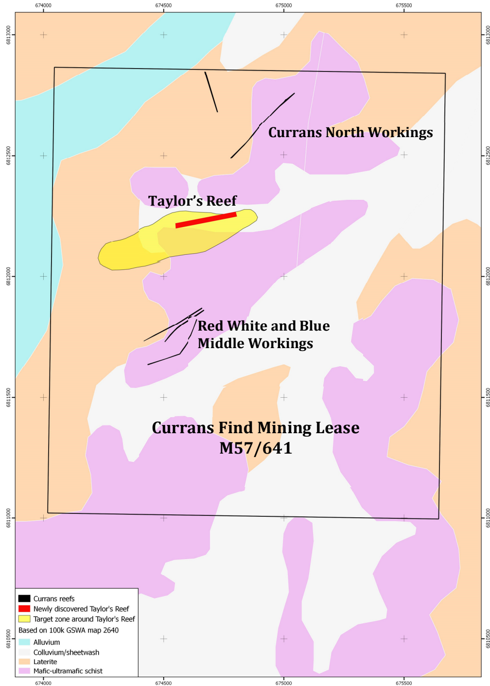
Figure 2. Surface Geology and the location of mineralised Quartz Reefs
