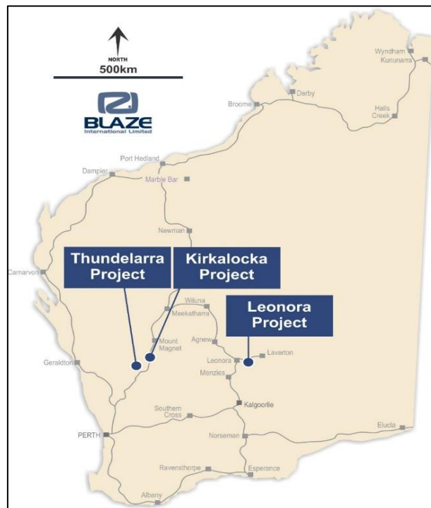
Figure 1. Location of the Kirkalocka, Thundelarra and Leonora Projects
