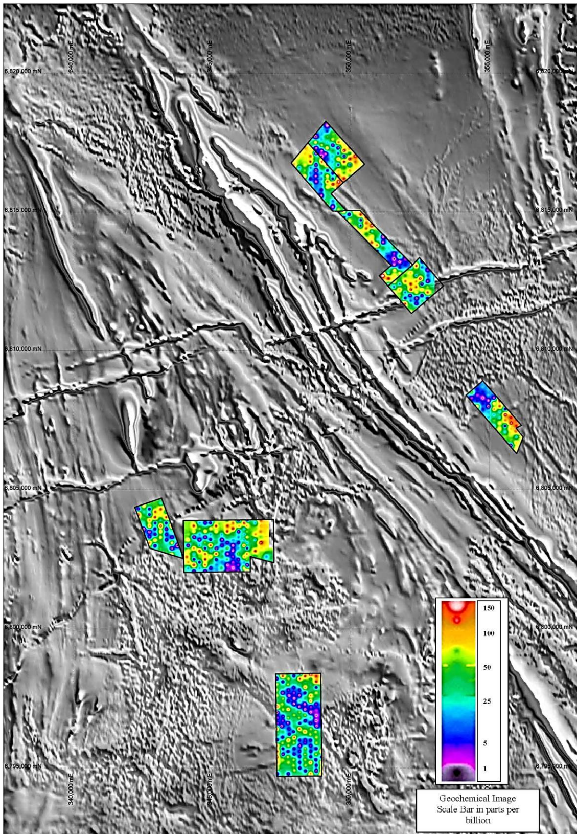
Figure 4. Leonora Project Ground: Imaged Gold Geochemistry on Magnetics
