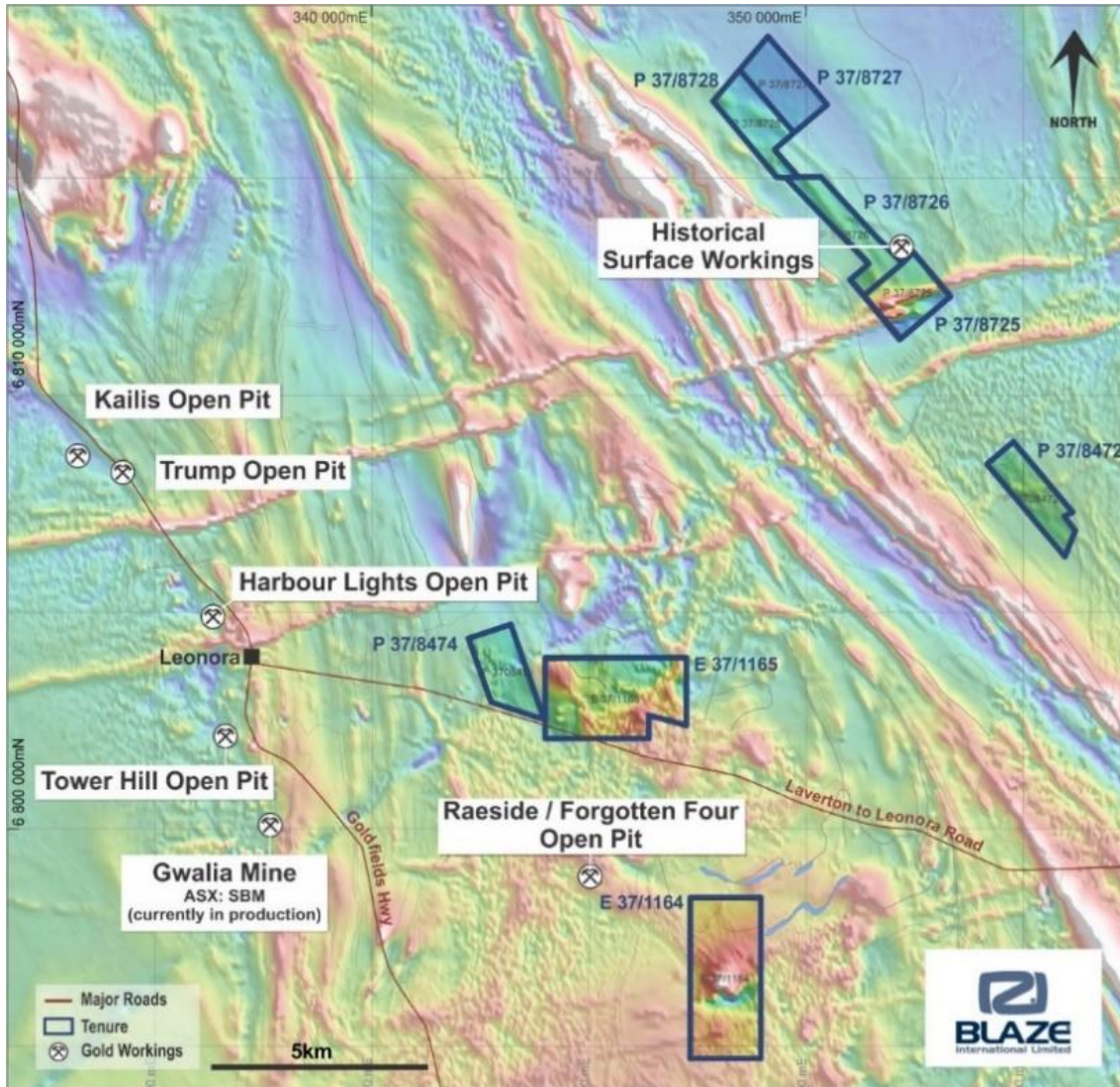
Figure 2. Leonora Project Ground
