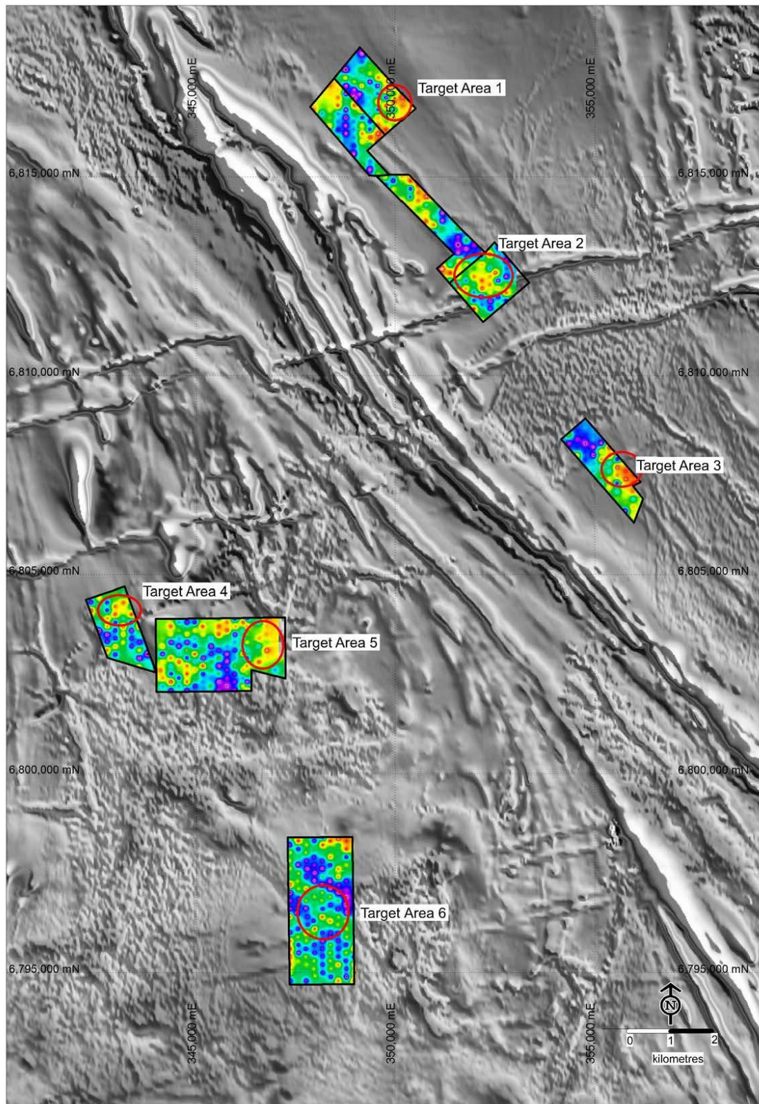
Figure 5. Leonora Project Ground: Imaged Gold Geochemistry and Targets on Magnetics
