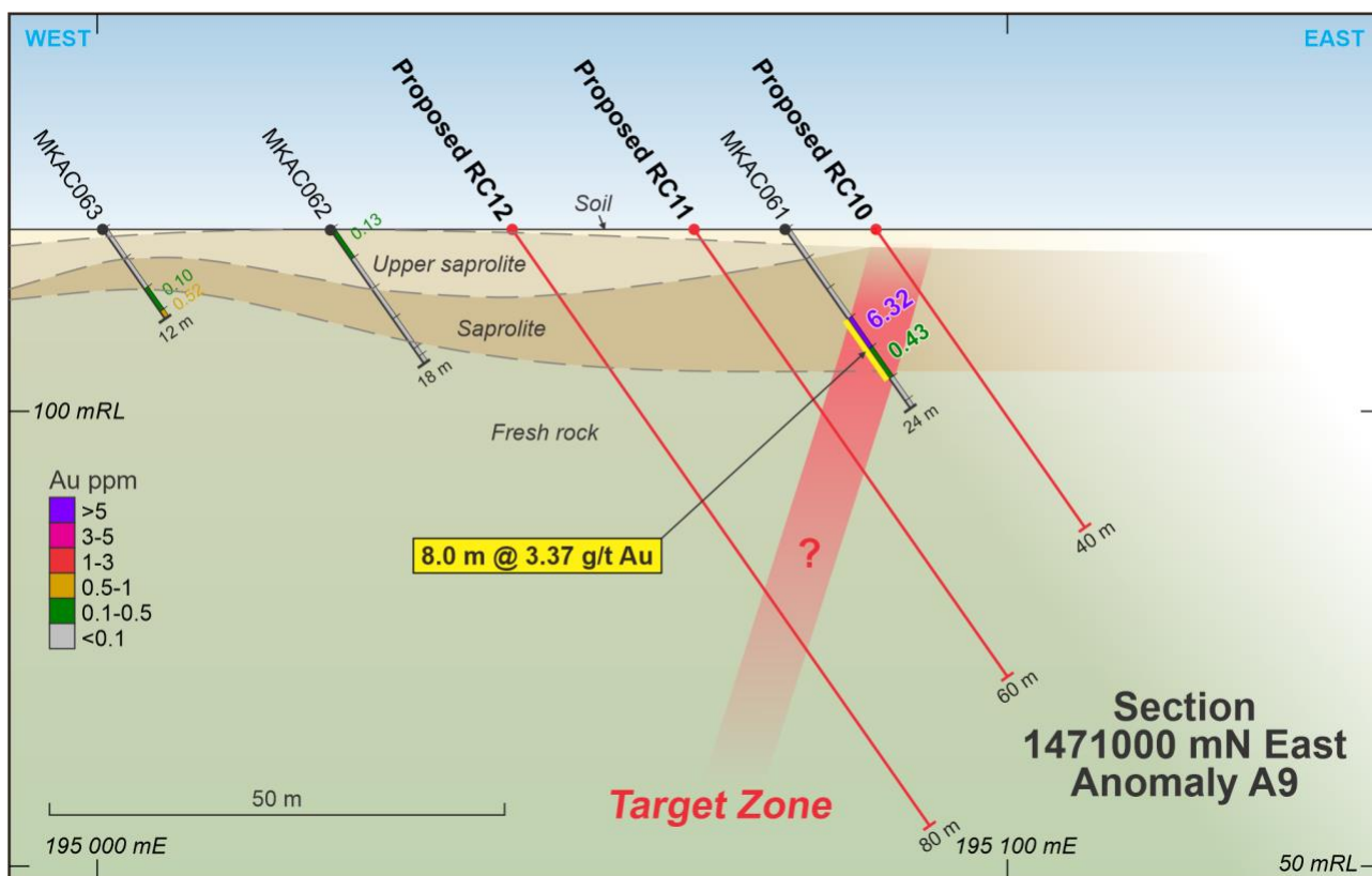
Figure 5 – Planned drilling at anomaly A9
