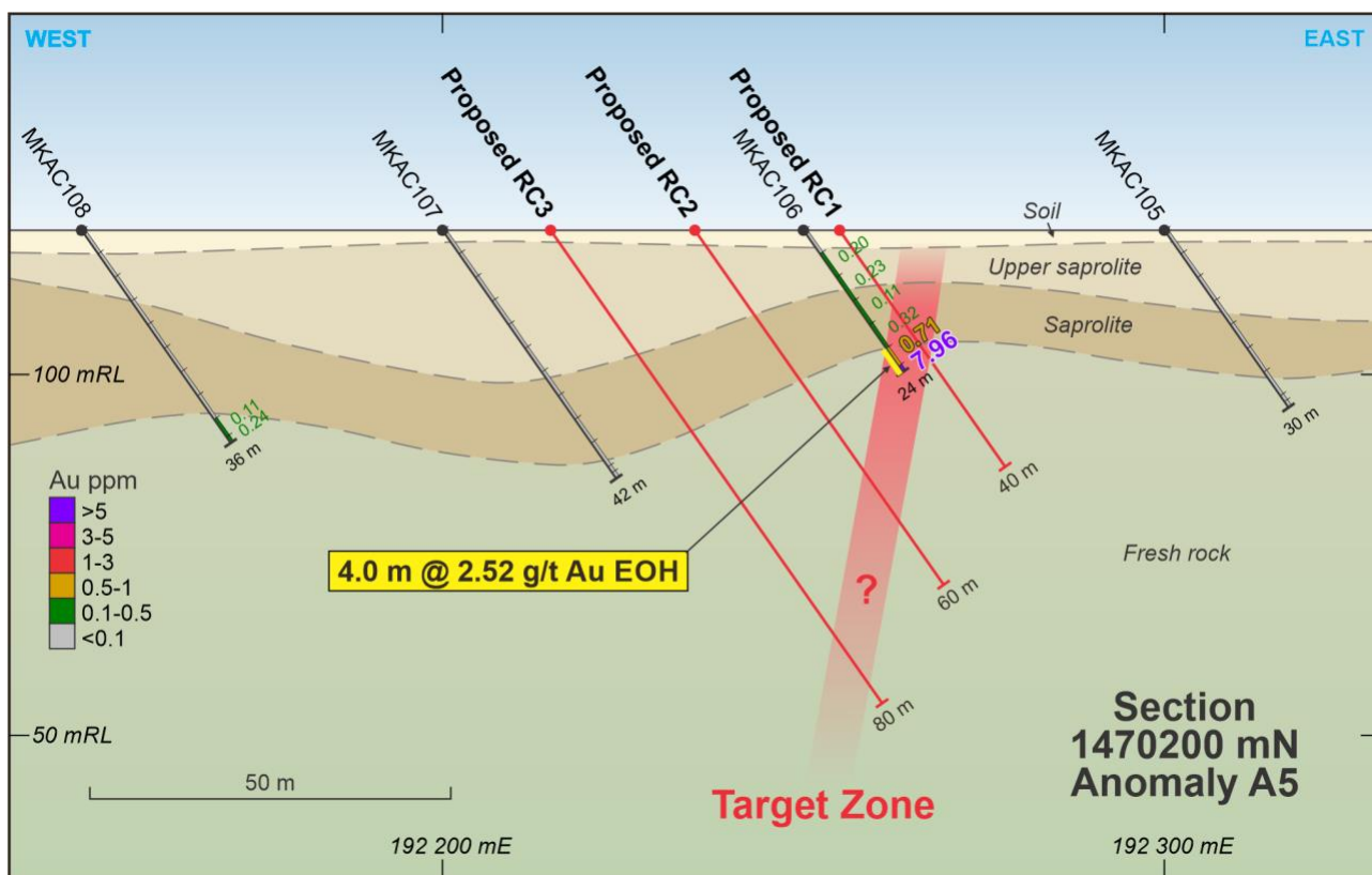
Figure 4 – Planned drilling at anomaly A5
