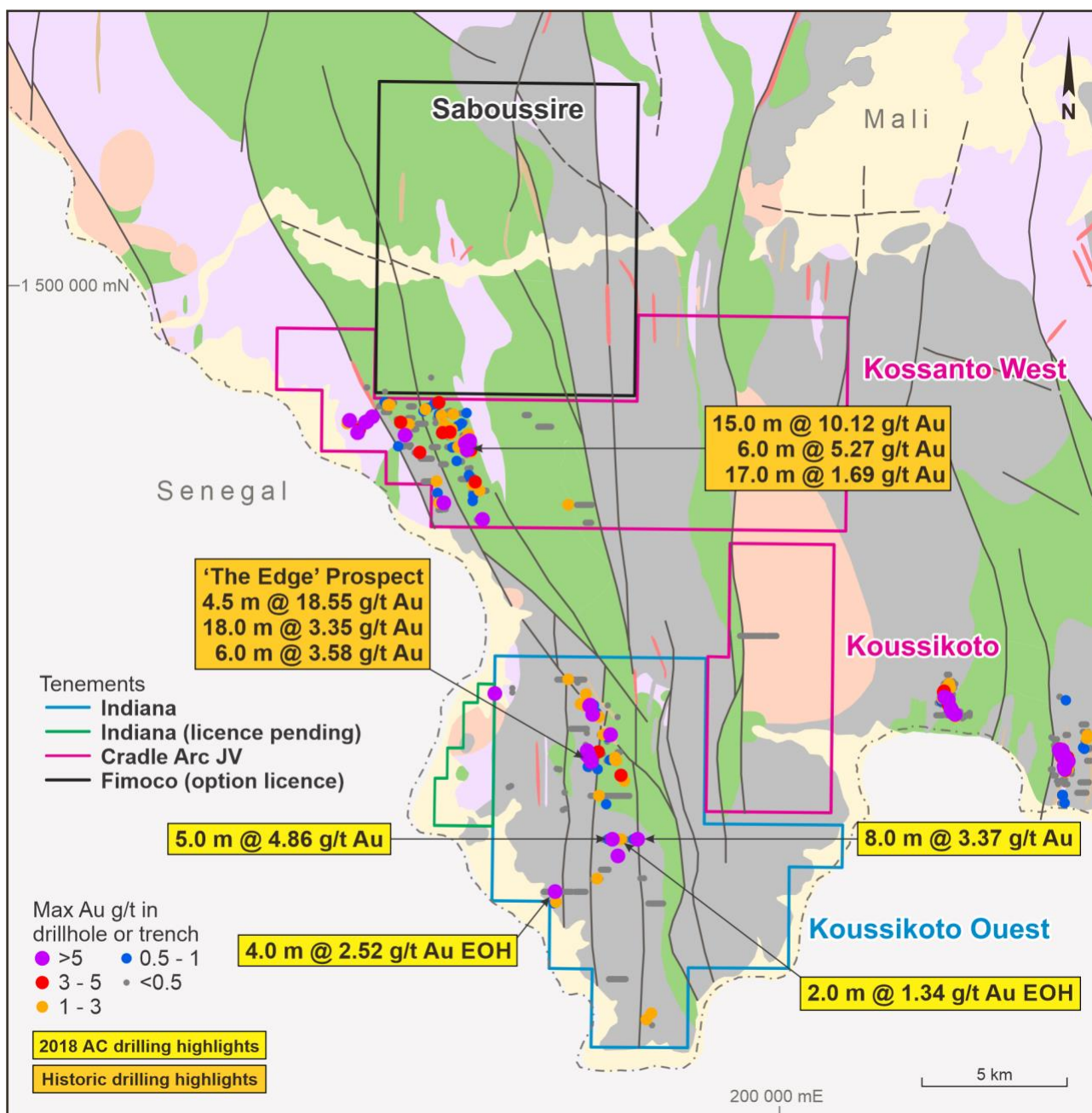
Figure 2 –Indiana West Mali Gold Project showing results of previous drilling and sampling programmes. Results relating to Kossanto Ouest – see ASX release – 11 September 2018
