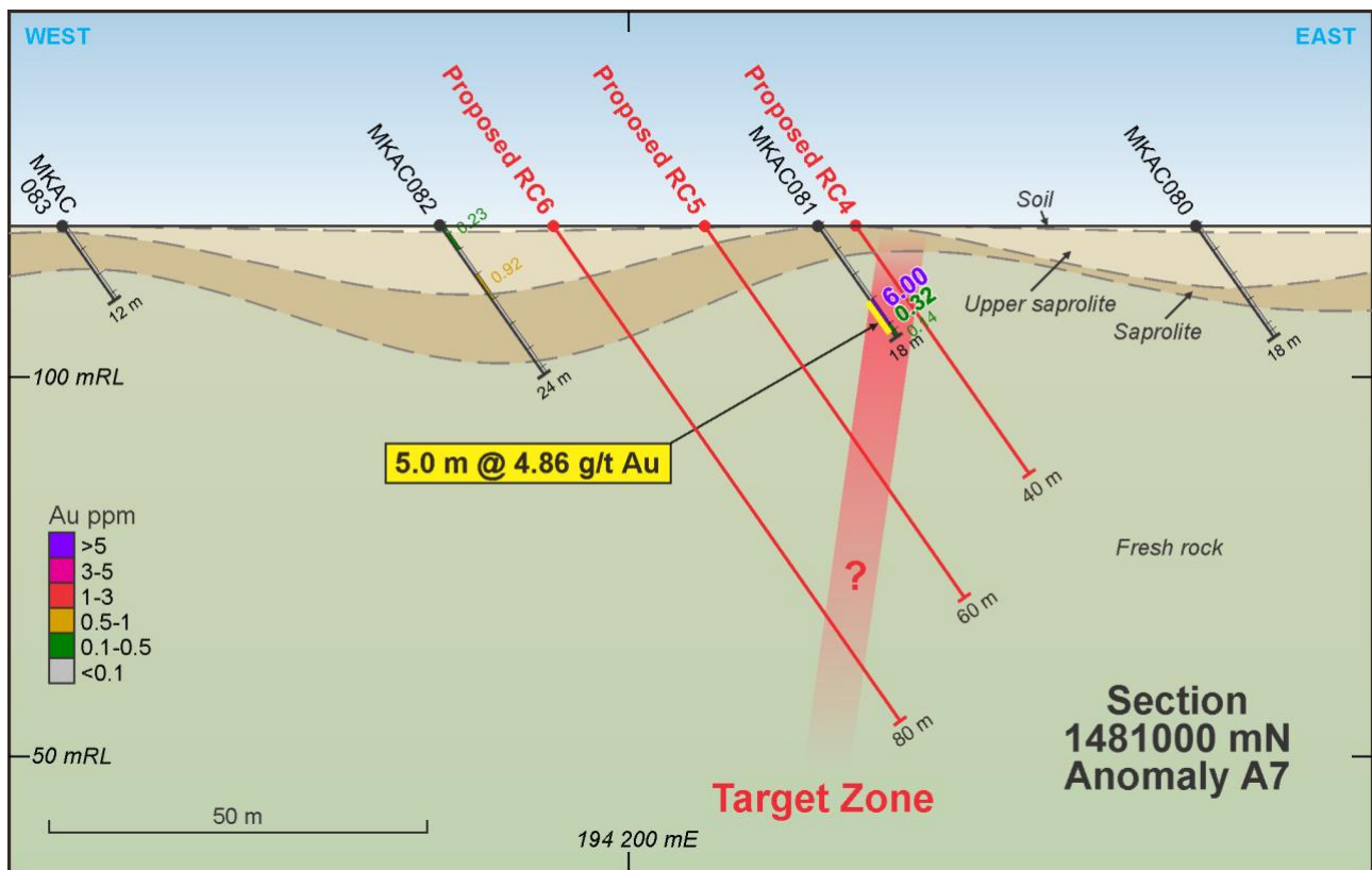
Figure 6 – Planned drilling at anomaly A7
