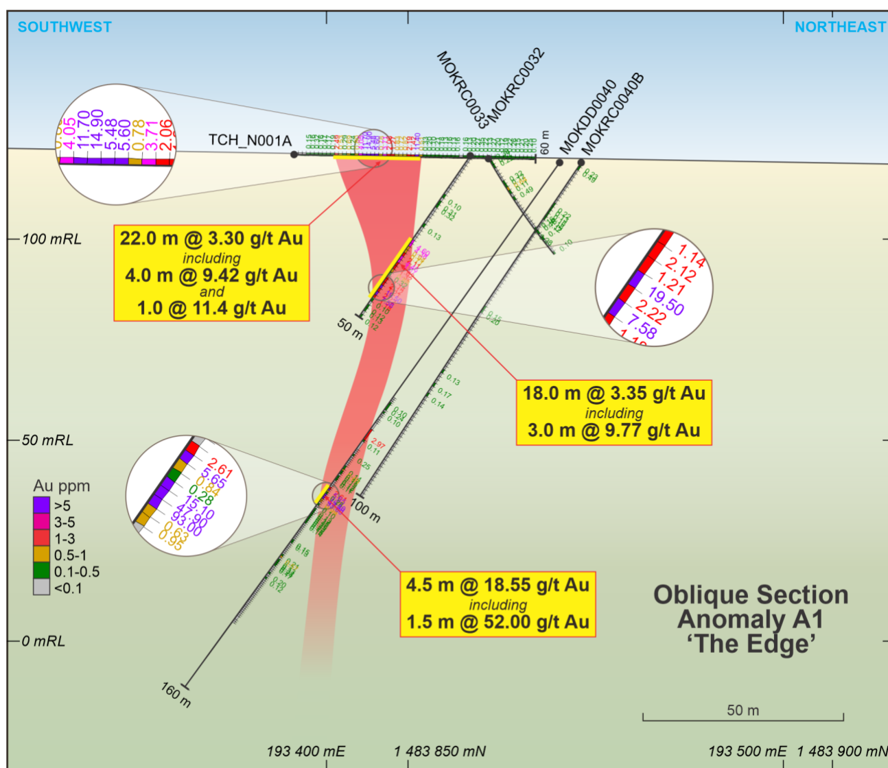
Figure 7 – Oblique section through “The Edge”
