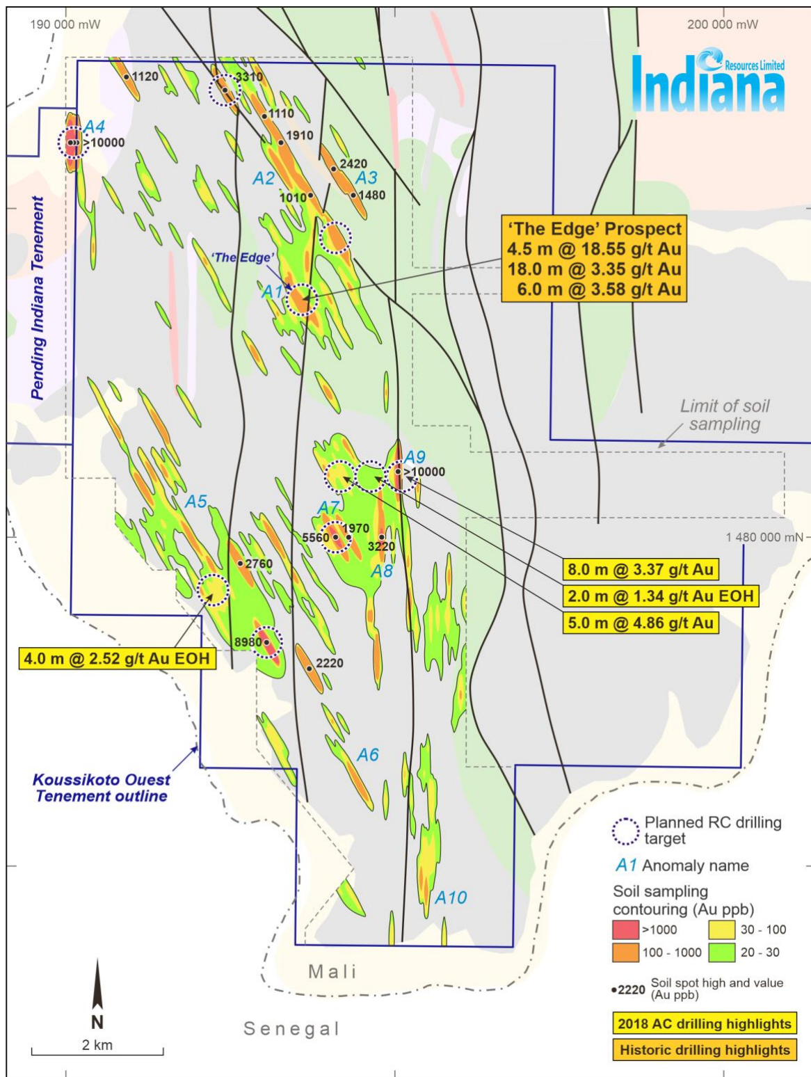
Figure 3 – Koussikoto Ouest - soil geochemical anomalies and planned drilling targets.
