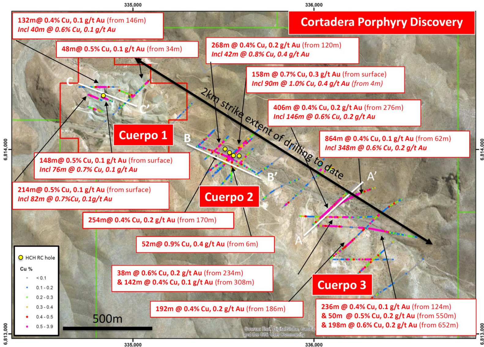
Figure 3 Plan view across the Cortadera discovery area displaying significant historical copper-gold DD intersections across Cuerpo 1, 2 and 3 tonalitic porphyry intrusive centres.
