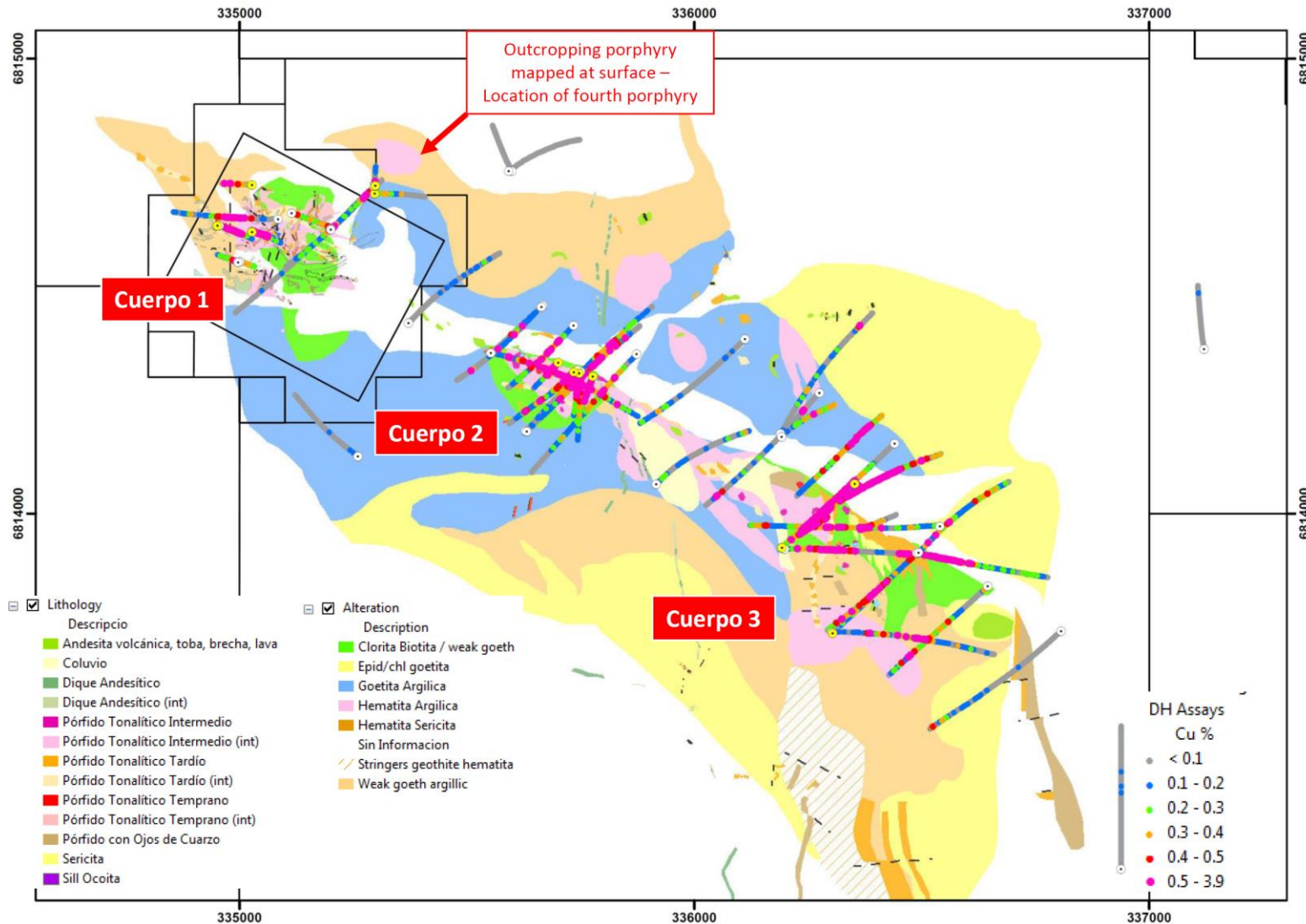
Figure 4 Plan view across the Cortadera discovery area displaying significant historical copper-gold DD intersections in relation to recently secured historical surface geology and alteration mapping.
