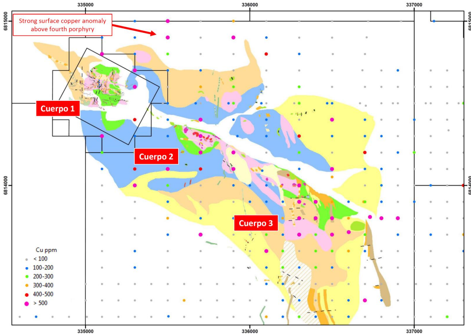
Figure 5 Plan view across the Cortadera discovery area displaying recently secured historical surface geology and alteration mapping in relation to historical surface geochemical survey copper results.
