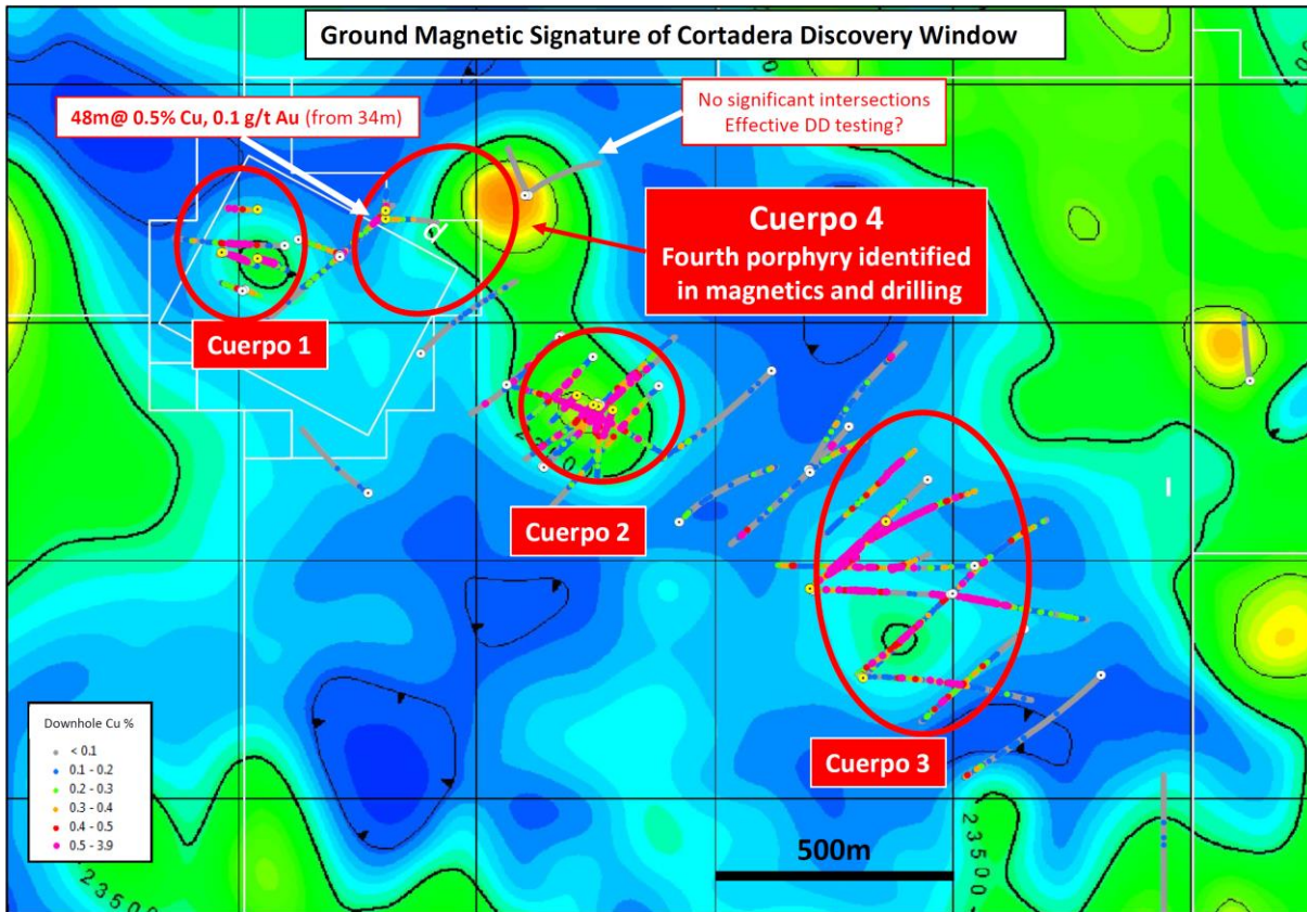
Figure 2 Ground Magnetic features within the Cortadera discovery window
