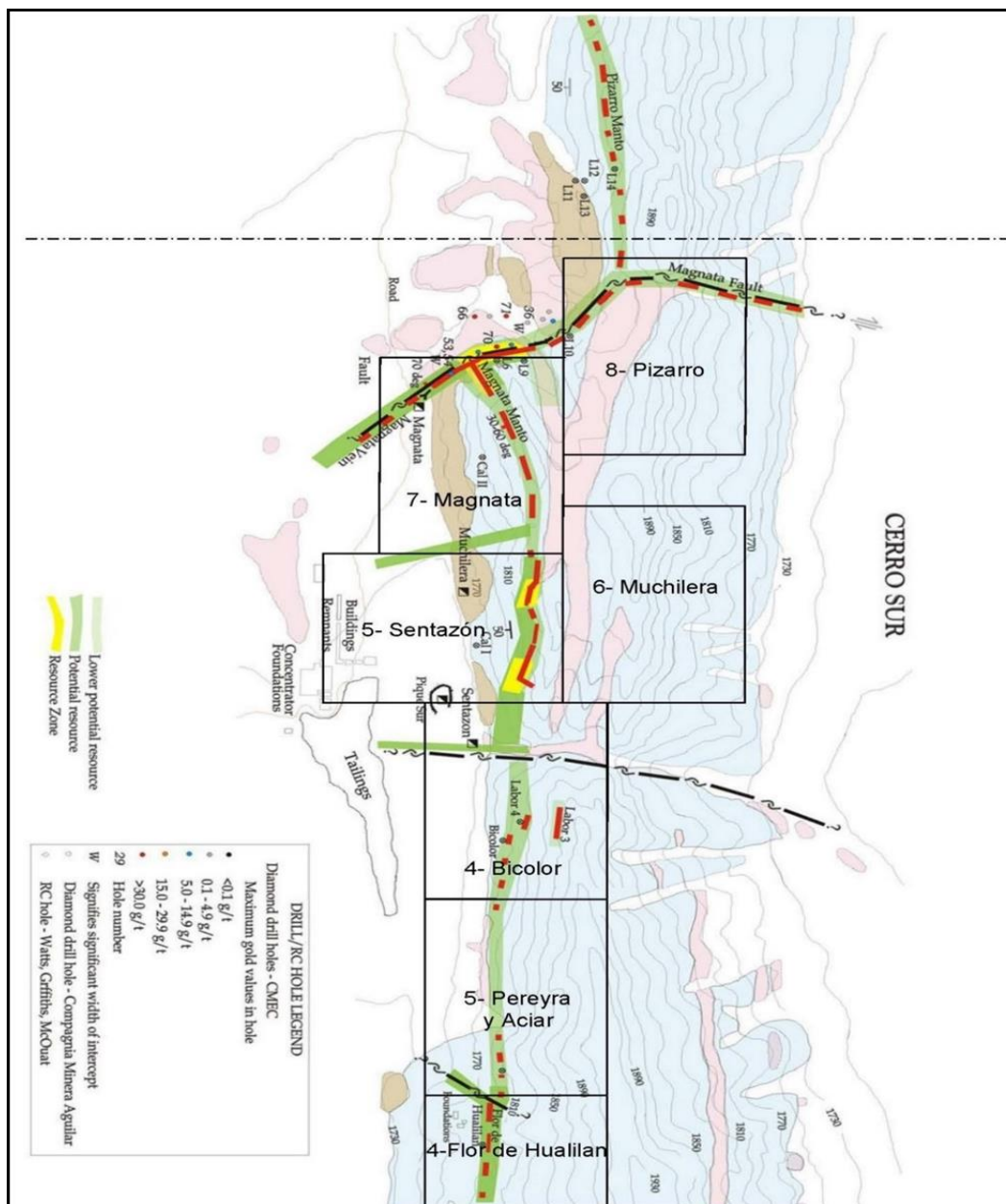
Figure 4 – Showing Main Cerro Sur Mineralised Zones (Source SRK Independent Geologist Report)
