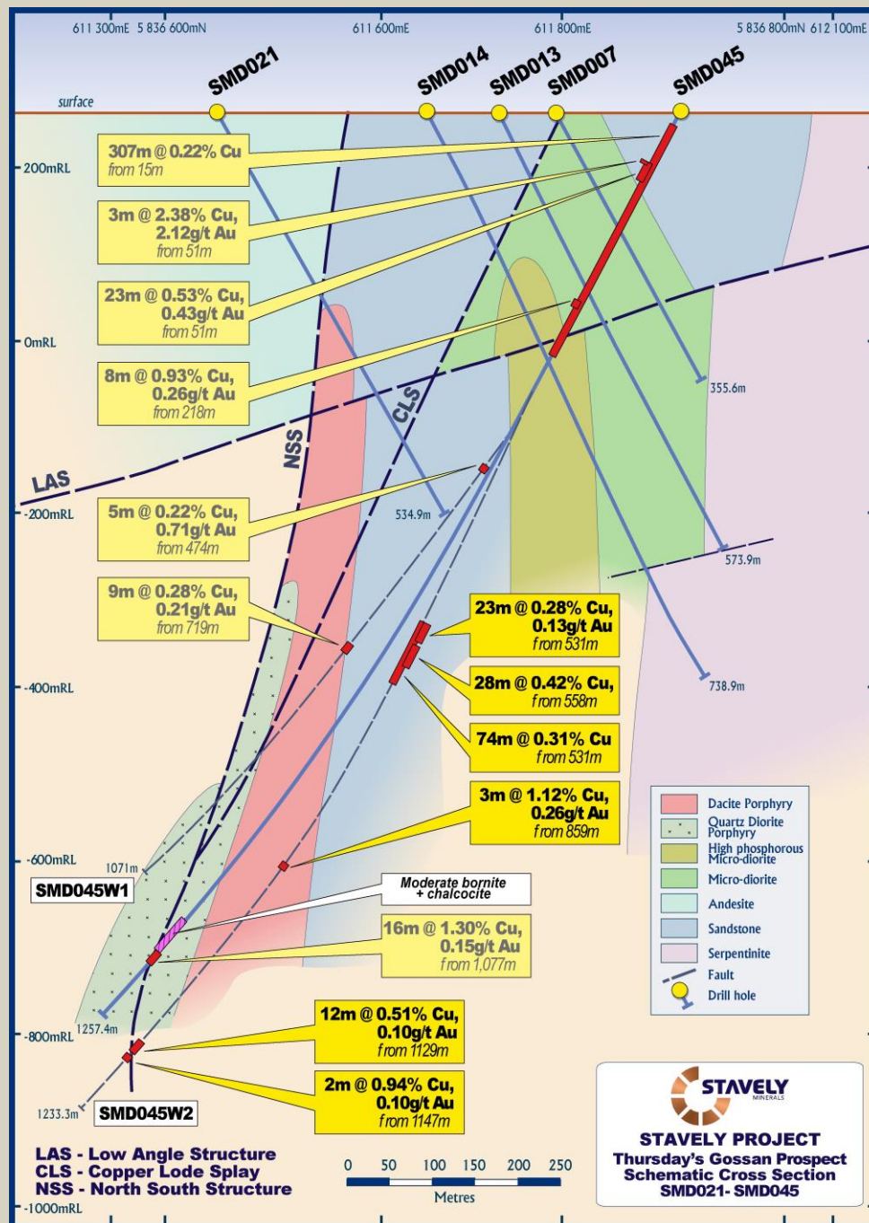
Figure 4. SMD045 drill section.
