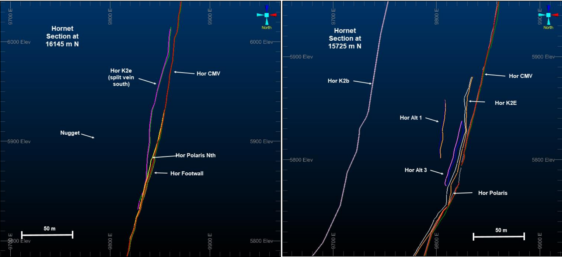
Figure 2. Cross section views of Hornet ore lodes
