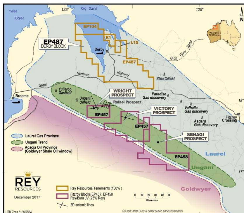
Figure 1. Location of the Derby Block and Rey's other oil and gas interests in the Canning Basin.
