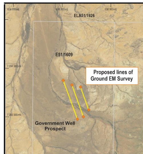
Figure 2. Location plan of the Government Well copper-silver-gold prospect and proposed Ground EM survey lines
