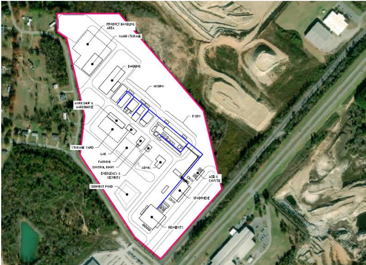
Figure 14 – Indicative Site Plan of Piedmont's Proposed 22,700 t/y Lithium Hydroxide Plant
