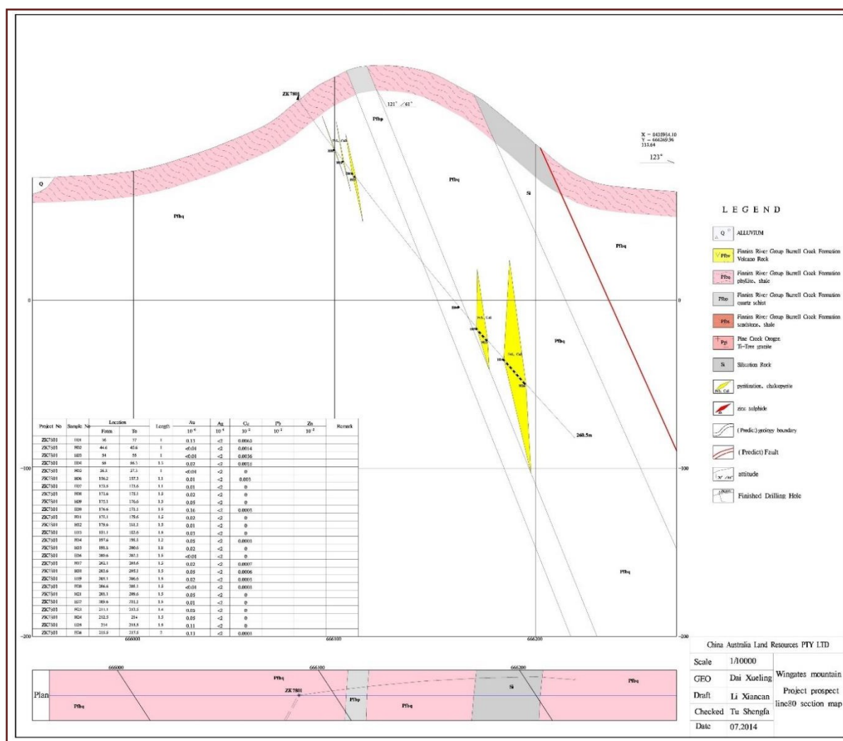
Figure 14: Cross section hole ZK7801
