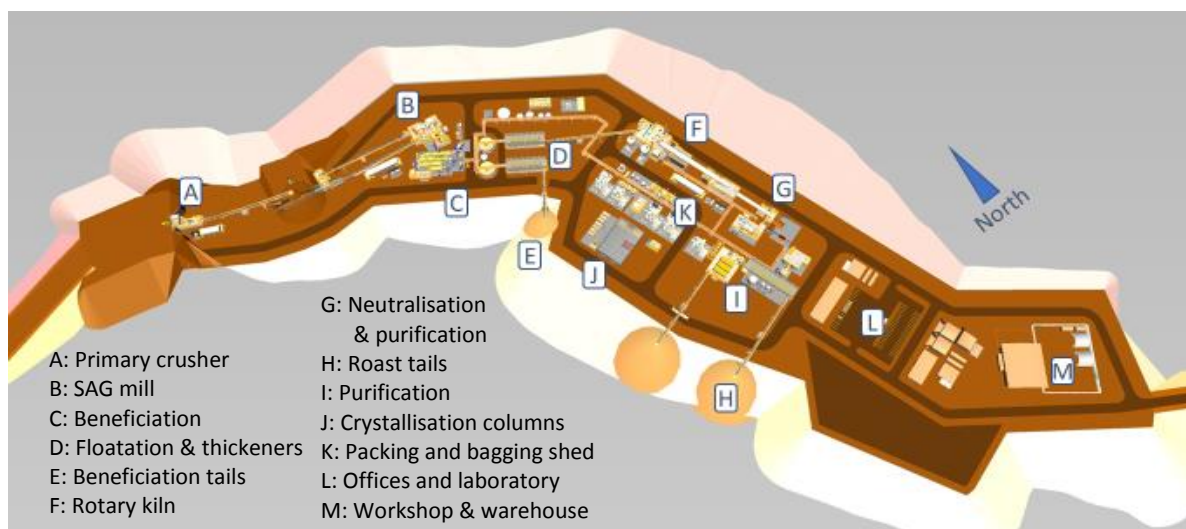
FIGURE 11: SAN JOSÉ AERIAL OVERVIEW OF THE PROCESSING PLANT
