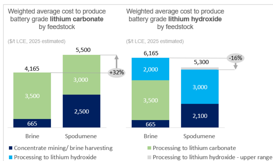
FIGURE M: ROCK RESOURCE PROVIDES ADVANTAGEOUS PROCESSING ROUTE
