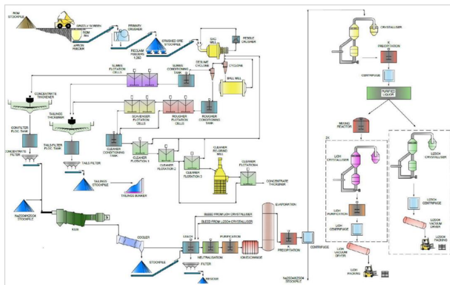
FIGURE 10: SAN JOSÉ PROCESS FLOWSHEET
