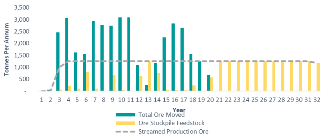
FIGURE 17: SAN JOSÉ LOM PRODUCTION PROFILE
