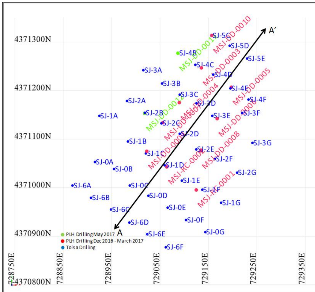
DRILL COLLAR PLAN OF SAN JOSE SHOWING TOLSA AND INFINITY (PREVIOUSLY PLYMOUTH: PLH) DRILLING. SECTION LINE A-A' AS SHOWN IN FIGURE 1A AND 1B.
