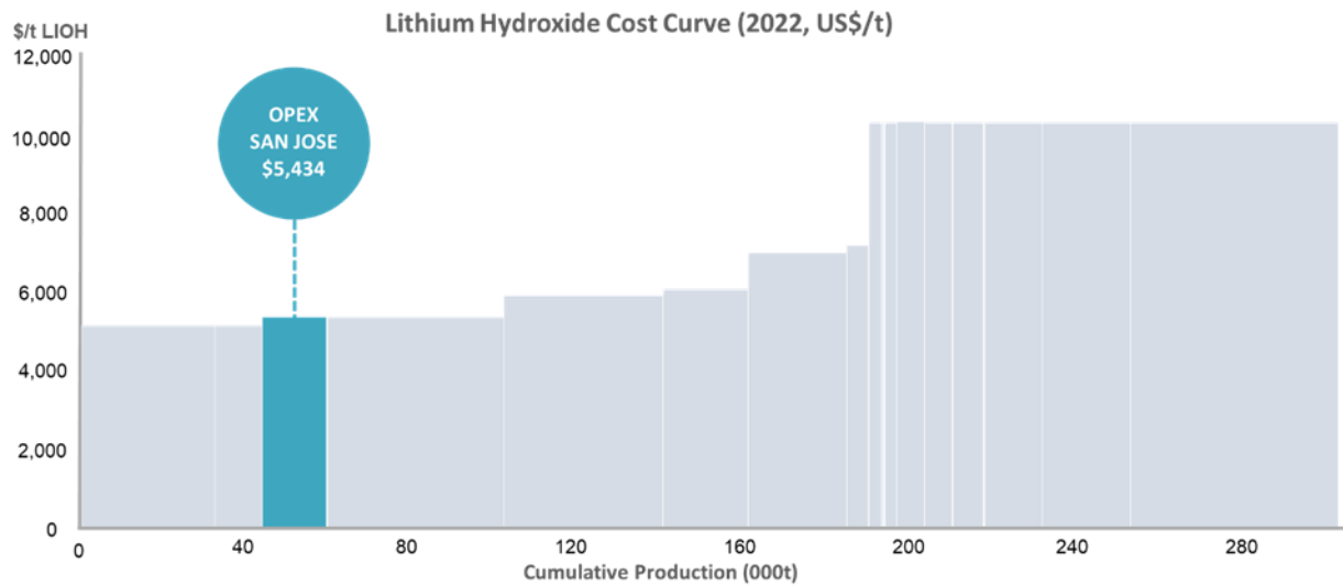
FIGURE N: LITHIUM HYDROXIDE COST CURVE 2022
