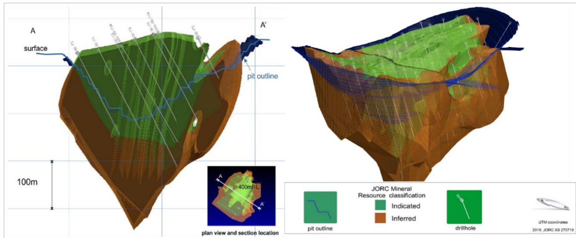
FIGURE 9: SAN JOSE PIT, RESOURCES AND DRILLING IN CROSS SECTION AND 3D VIEW
