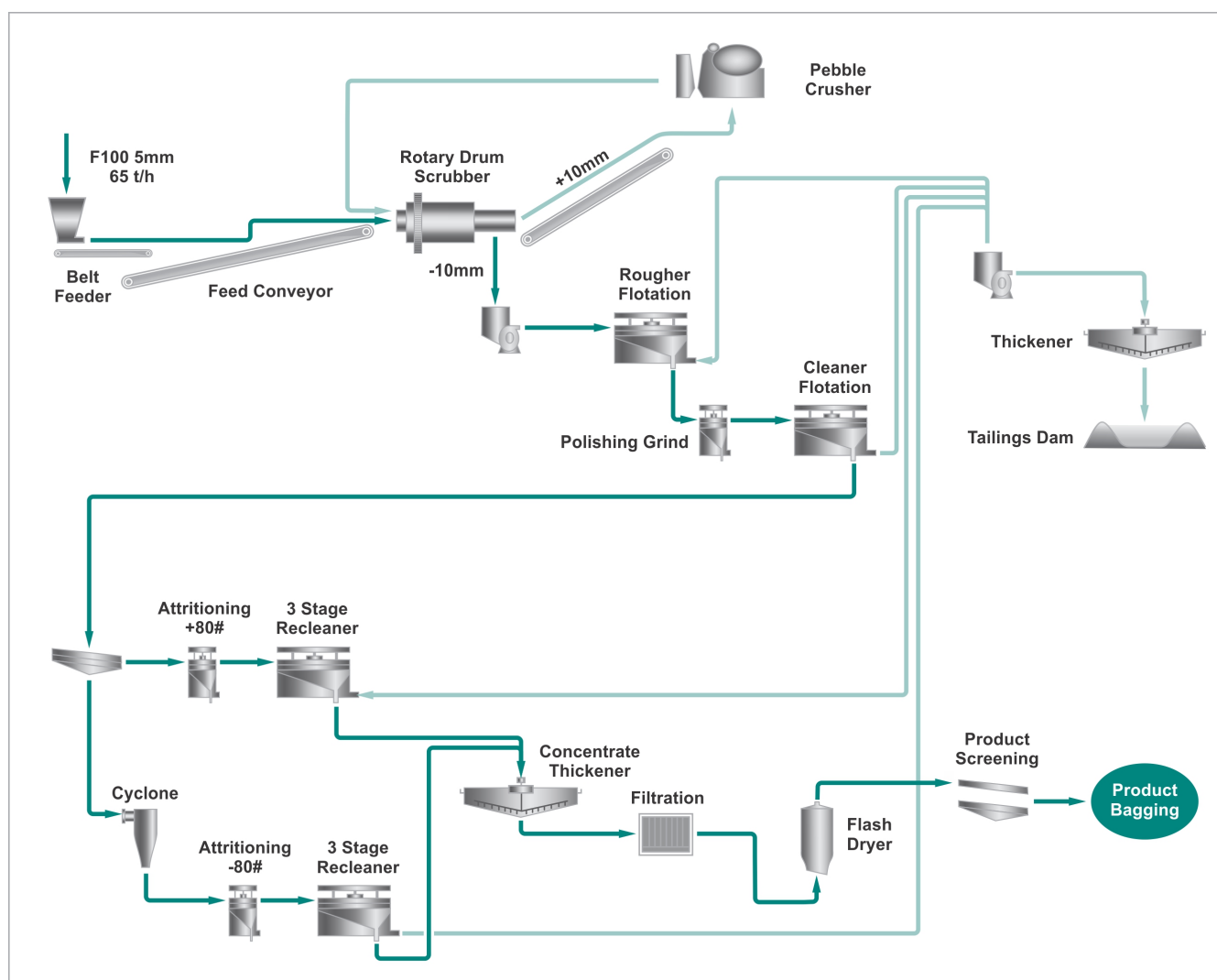
Figure 2: Simplified process flowsheet for Malingunde.
