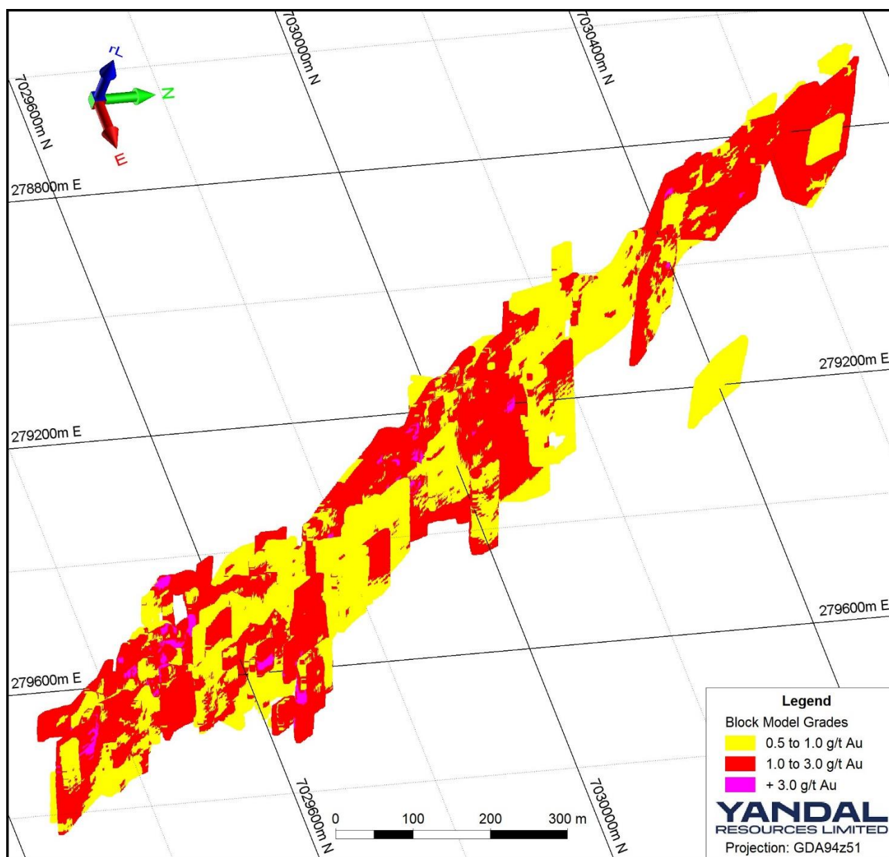
Figure 1 – Three-dimensional longitudinal representation of the September 2019 Flushing Meadows initial Mineral Resource Estimate block model by grade range.
