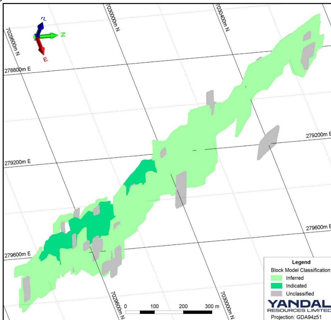
Figure 7 – Flushing Meadows Mineral Resource Estimate block model Resource Classification, oblique view.
