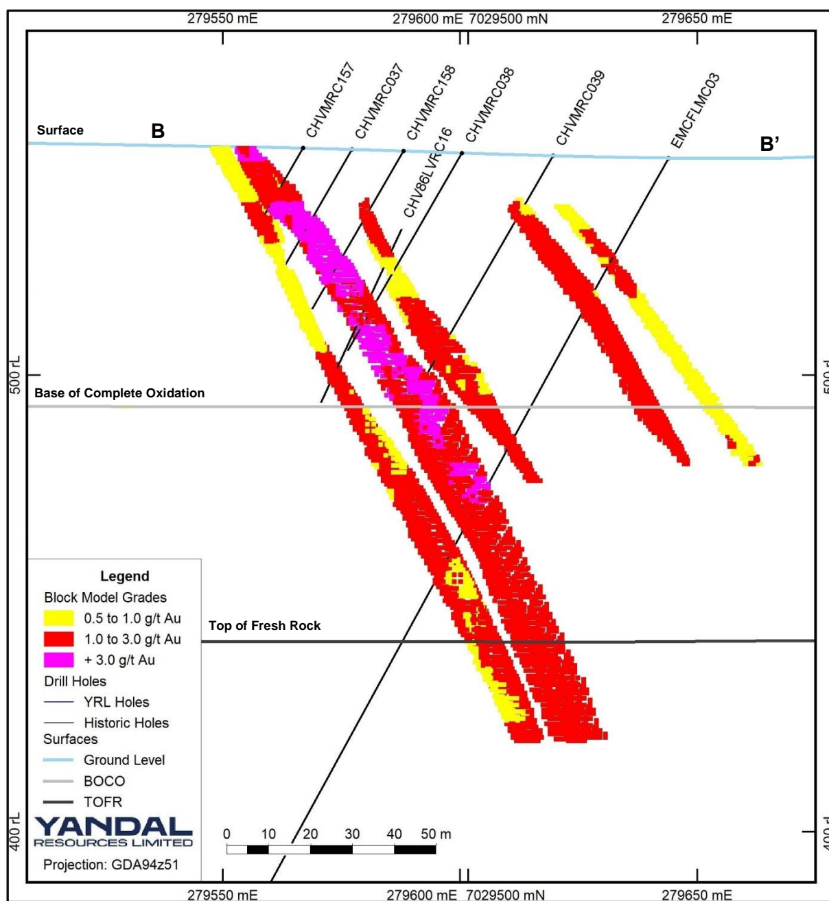
Figure 6 – Flushing Meadows Mineral Resource Estimate block model cross section B – B' by grade range with drill hole traces and weathering surfaces.
