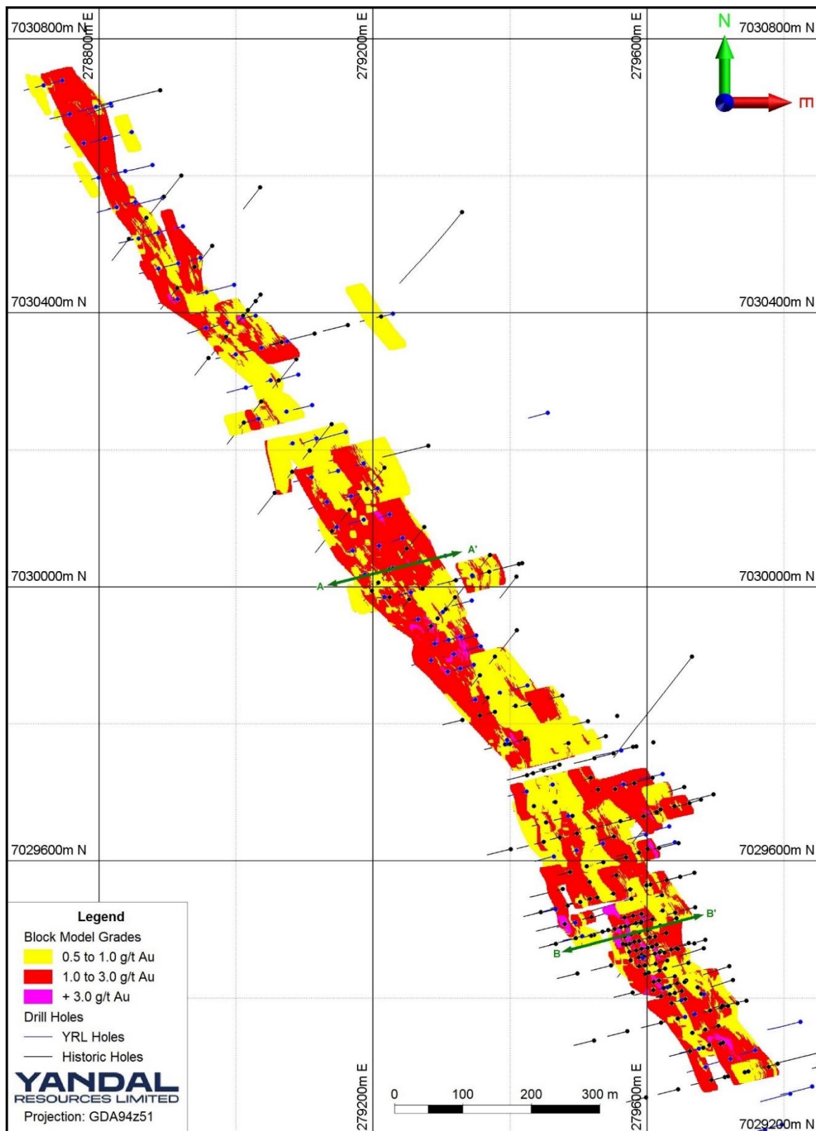
Figure 4 – Flushing Meadows Mineral Resource Estimate block model by grade range with drill hole traces and the location of cross sections A - A' (Figure 5) and B - B' (Figure 6).
