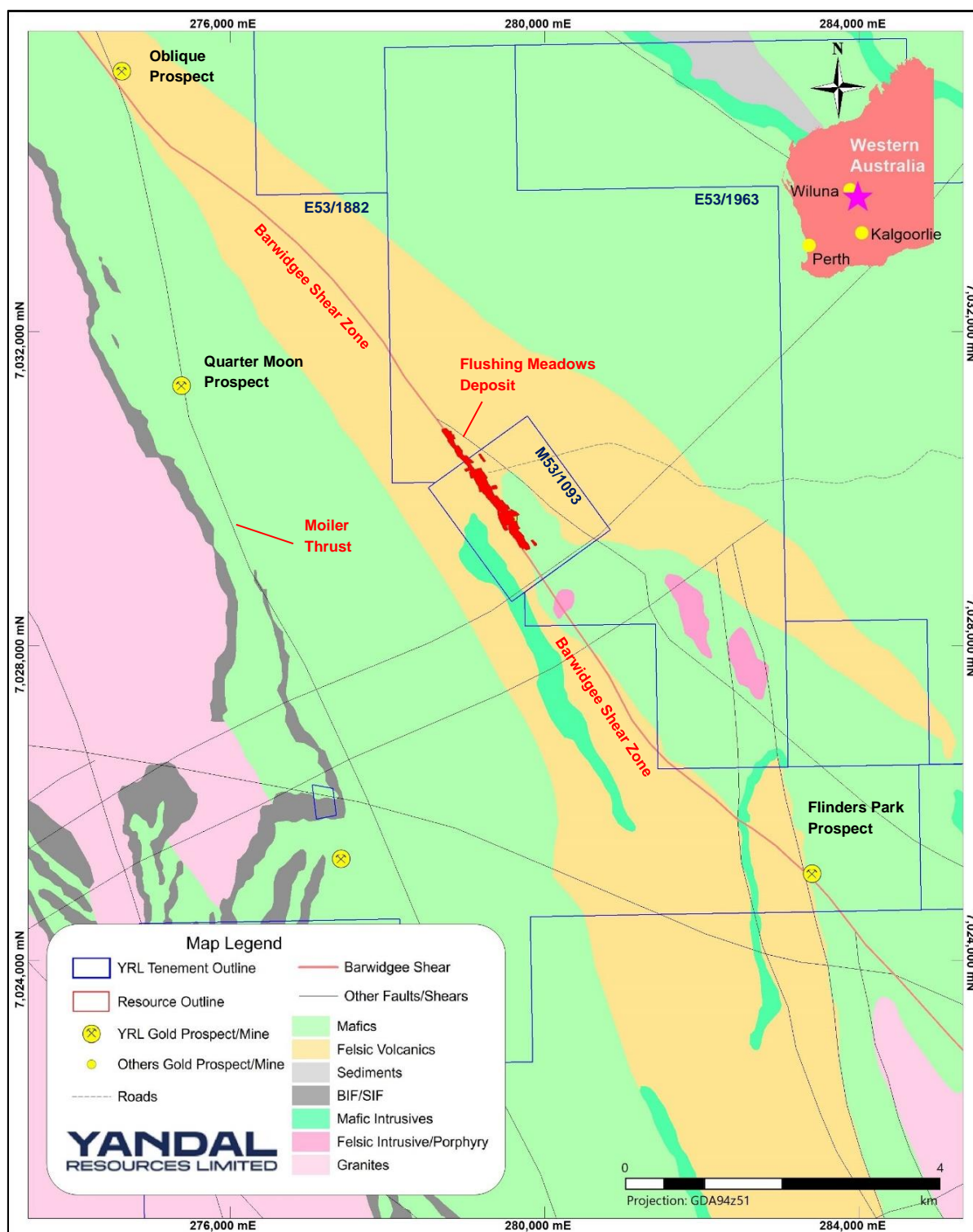
Figure 3 – Regional geology map showing major structures, the location of the Flushing Meadows deposit and mining tenements.
