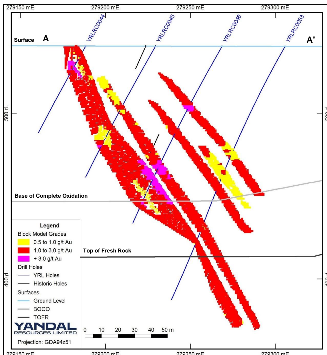
Figure 5 – Flushing Meadows Mineral Resource Estimate block model cross section A – A' by grade range with drill hole traces and weathering surfaces.
