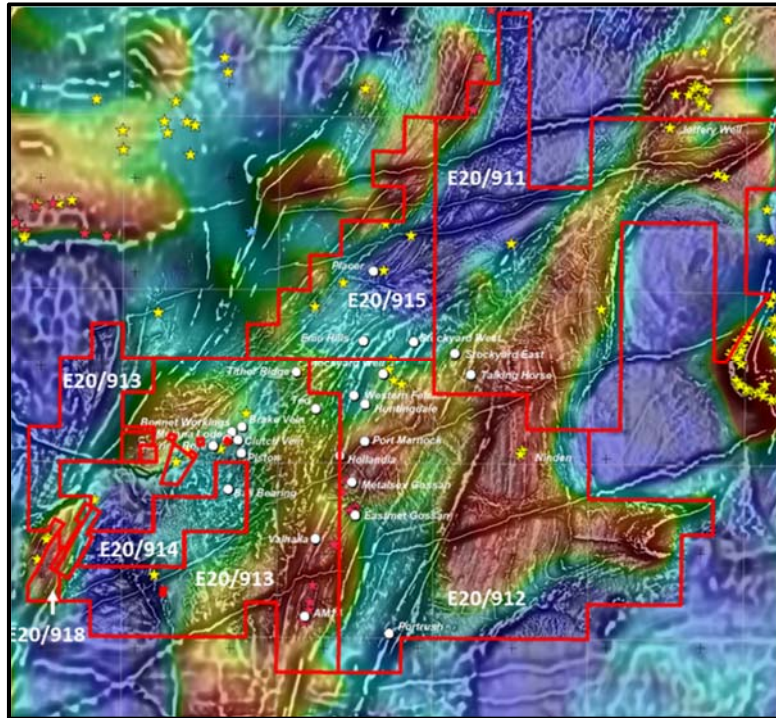
Figure 3. Murchison Project, Grey Scale 1 st VD Magnetic Imagery over Coloured Gravity VD1 Imagery with Metallogenic Data.
