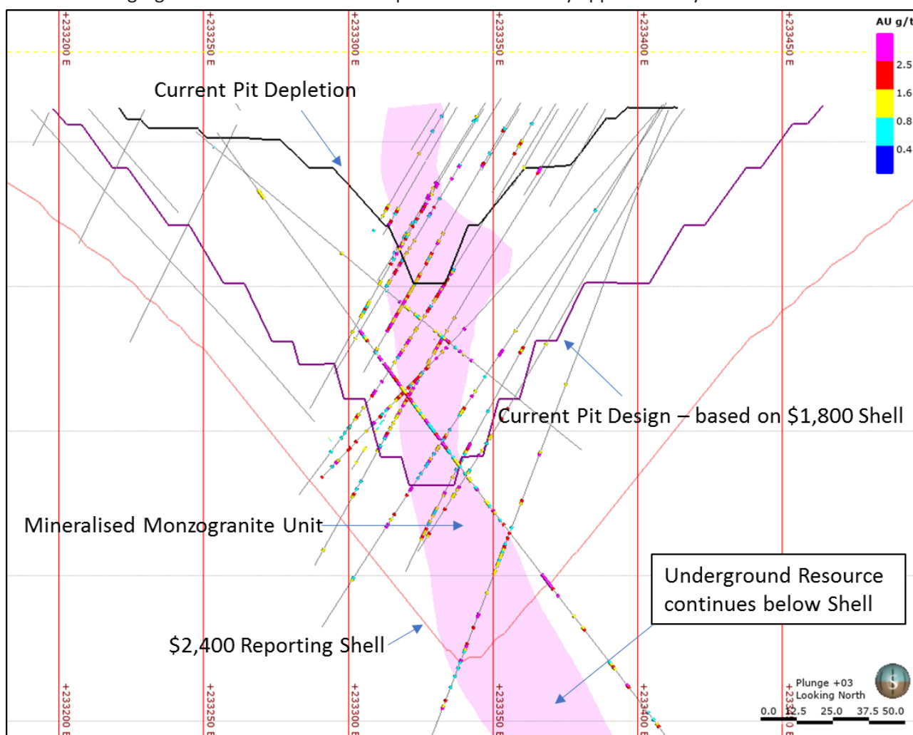
Figure 2. Williamson cross-section showing the mineralised monzogranite unit with the current pit design and the $2400 reporting shell.
