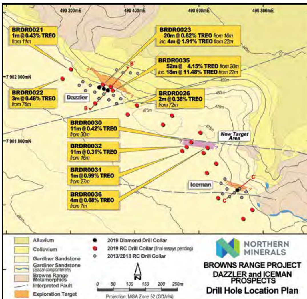
Brown's Range Project: Dazzler and Iceman Prospects - Drill Hole Location Plan
