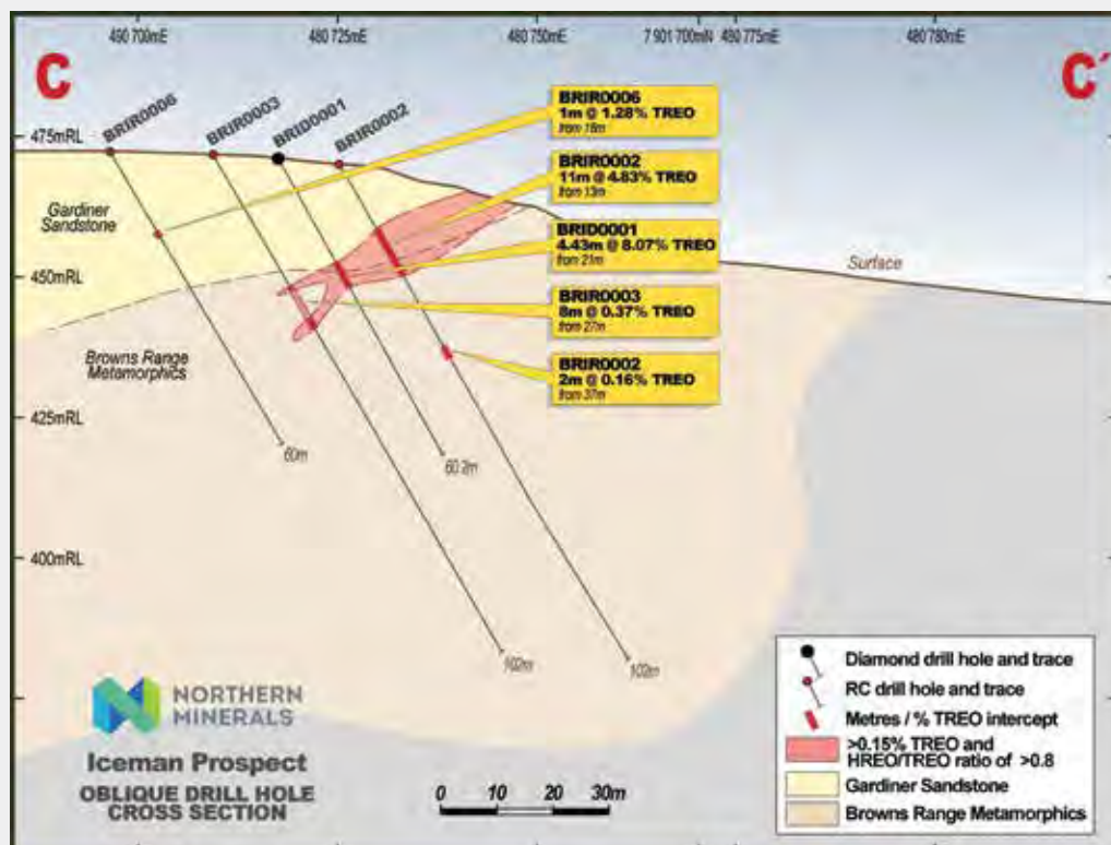
Brown's Range Project: Iceman Prospect - Oblique Drill Hole Cross Section
