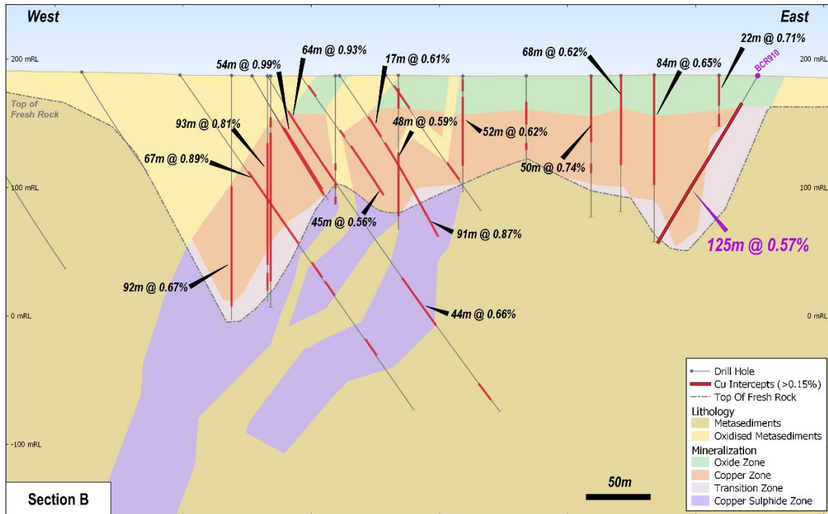
Figure 4 'Section B' through the Blackard deposit with new drill hole BCR910 (see Figure 2 for location)
