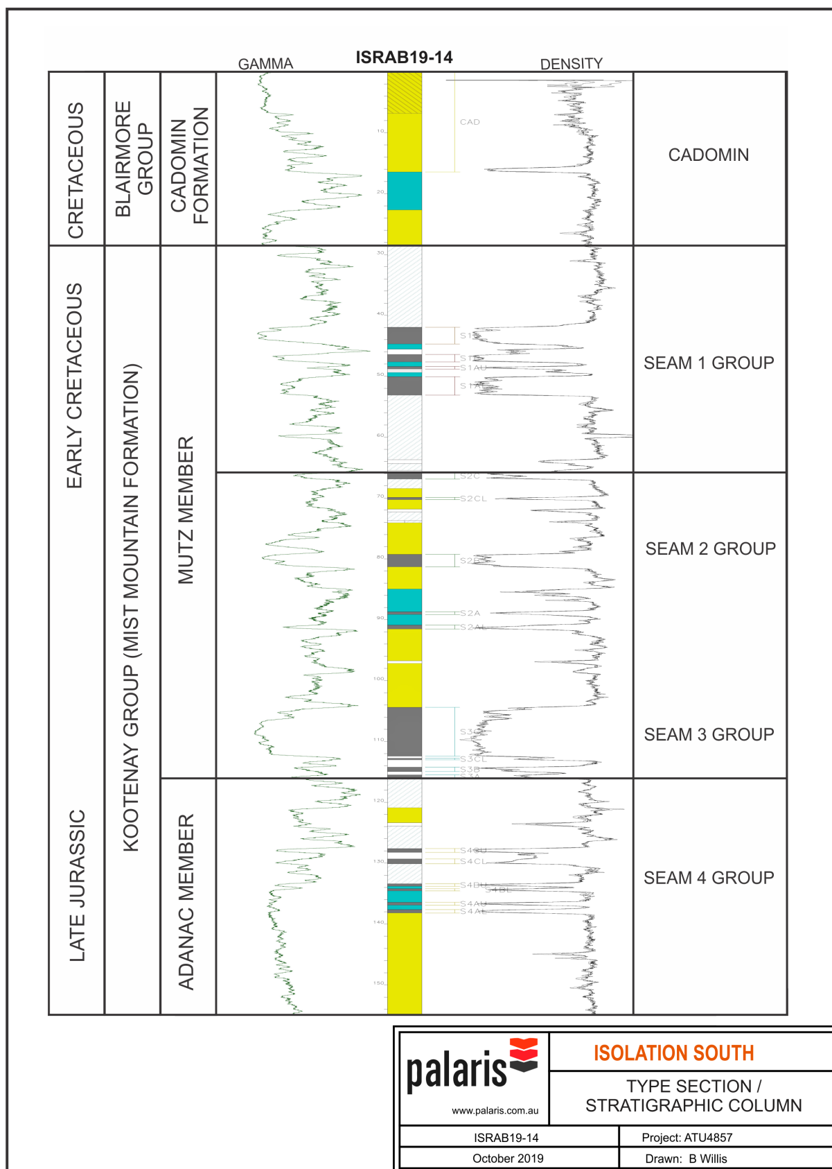
Figure 3: Isolation South stratigraphic column and type section from ISRAB19-14
