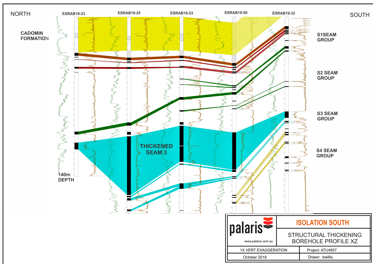
Figure 4: Borehole profile section (north-south) showing extent of seam thickening in Seam 3 group
