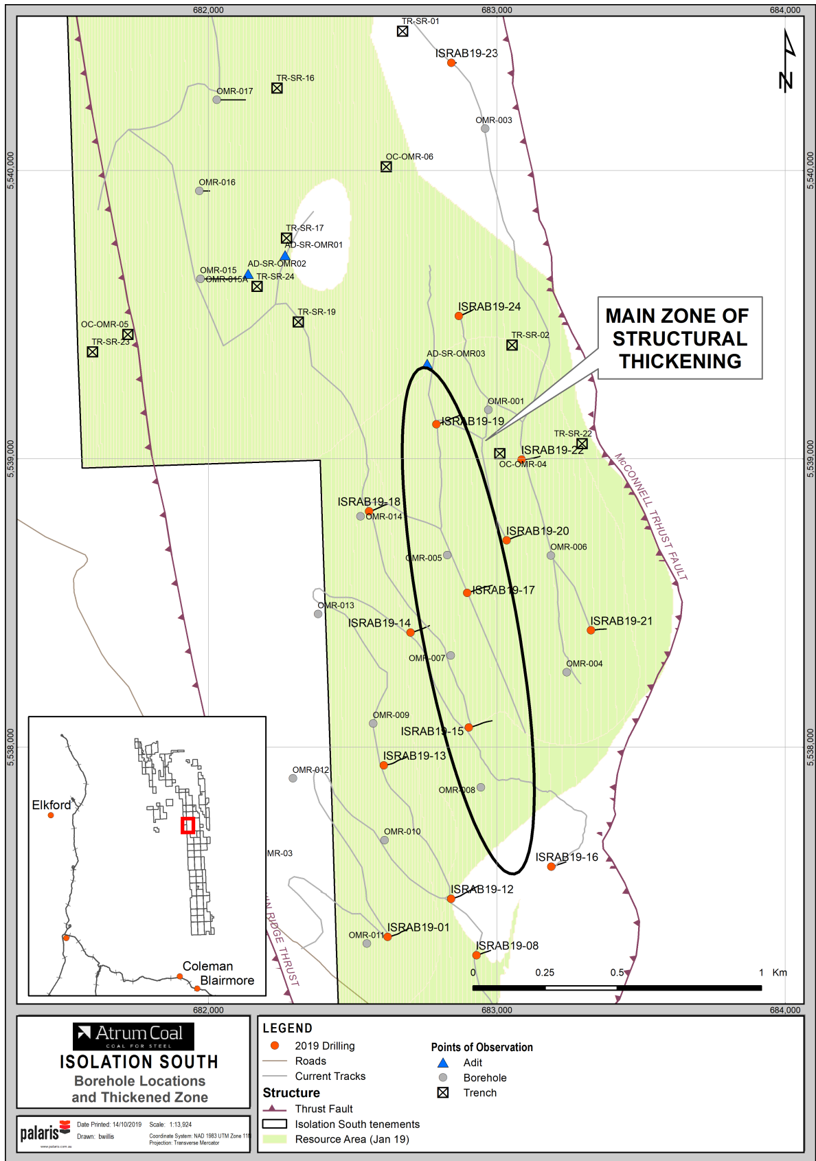
Figure 2: Completed drill hole locations and zone of structural thickening at Isolation South
